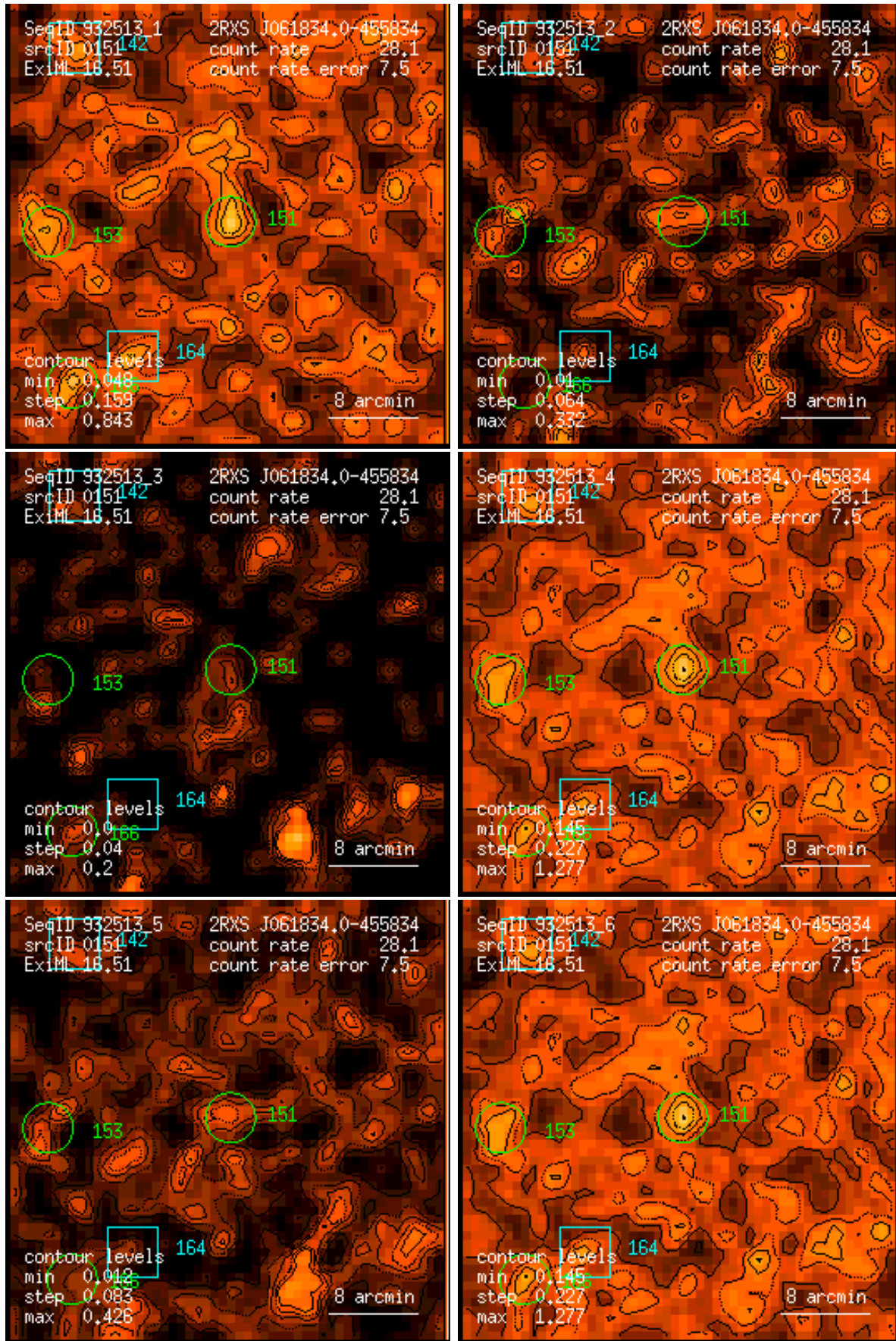
Figure 151: RASS 932513: detection 0151: band rate images, Gaussian filter: (1) PSPC channels 11 – 41, (2) 52 – 90, (3) 91 – 201, (4) 11 – 235, (5) 52 – 201, (6) 11 – 201. Broad band rates in counts/ks. Band rate contour levels in counts/ks/arcmin 2 .
