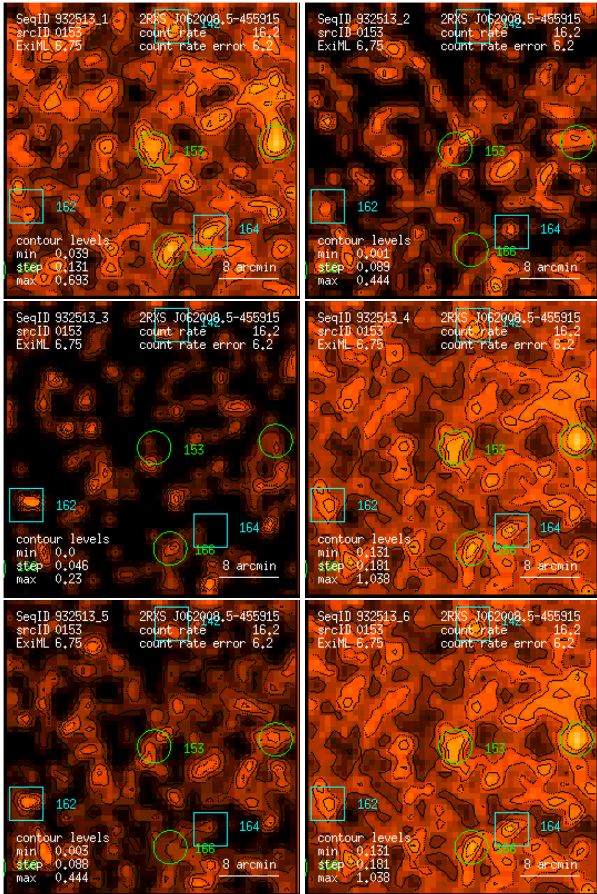
Figure 153: RASS 932513: detection 0153: band rate images, Gaussian filter: (1) PSPC channels 11 – 41, (2) 52 – 90, (3) 91 – 201, (4) 11 – 235, (5) 52 – 201, (6) 11 – 201. Broad band rates in counts/ks. Band rate contour levels in counts/ks/arcmin 2 .
