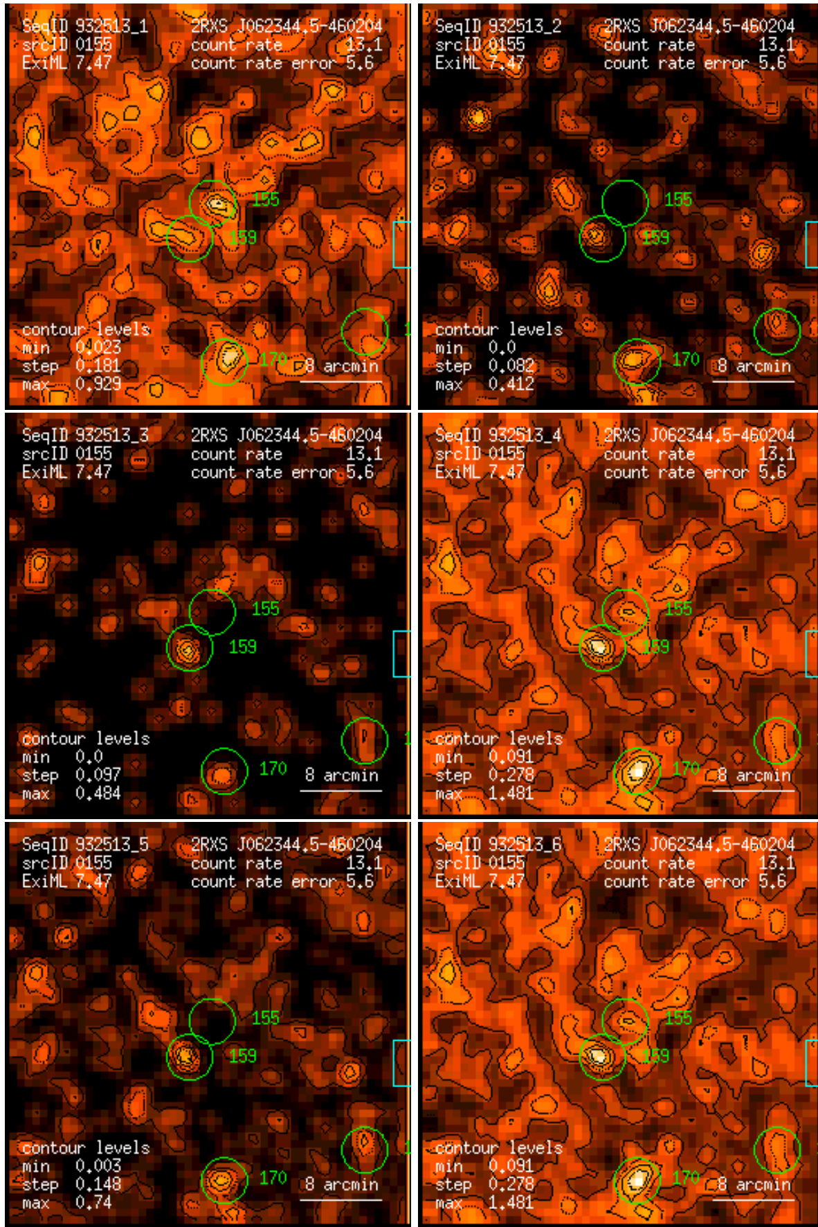
Figure 155: RASS 932513: detection 0155: band rate images, Gaussian filter: (1) PSPC channels 11 – 41, (2) 52 – 90, (3) 91 – 201, (4) 11 – 235, (5) 52 – 201, (6) 11 – 201. Broad band rates in counts/ks. Band rate contour levels in counts/ks/arcmin 2 .
