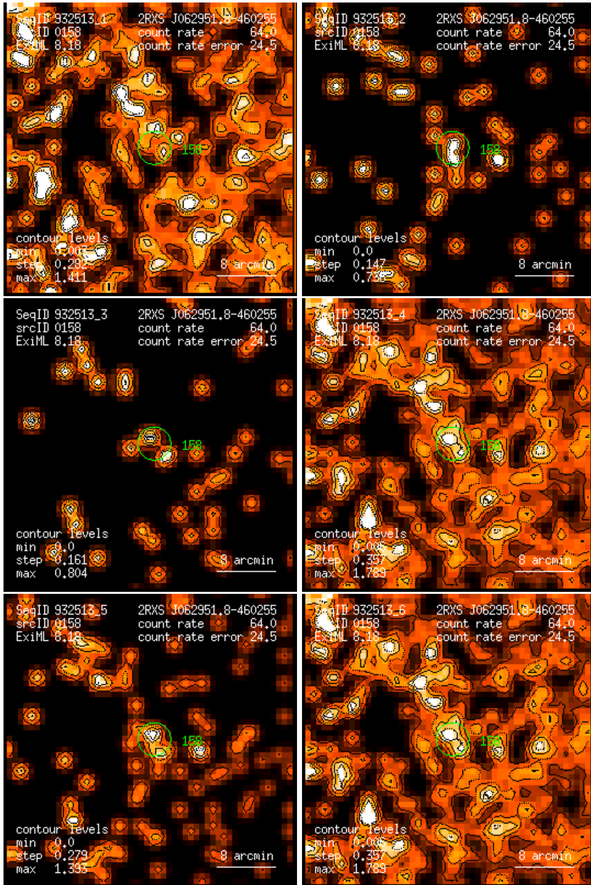
Figure 158: RASS 932513: detection 0158: band rate images, Gaussian filter: (1) PSPC channels 11 – 41, (2) 52 – 90, (3) 91 – 201, (4) 11 – 235, (5) 52 – 201, (6) 11 – 201. Broad band rates in counts/ks. Band rate contour levels in counts/ks/arcmin 2 .
