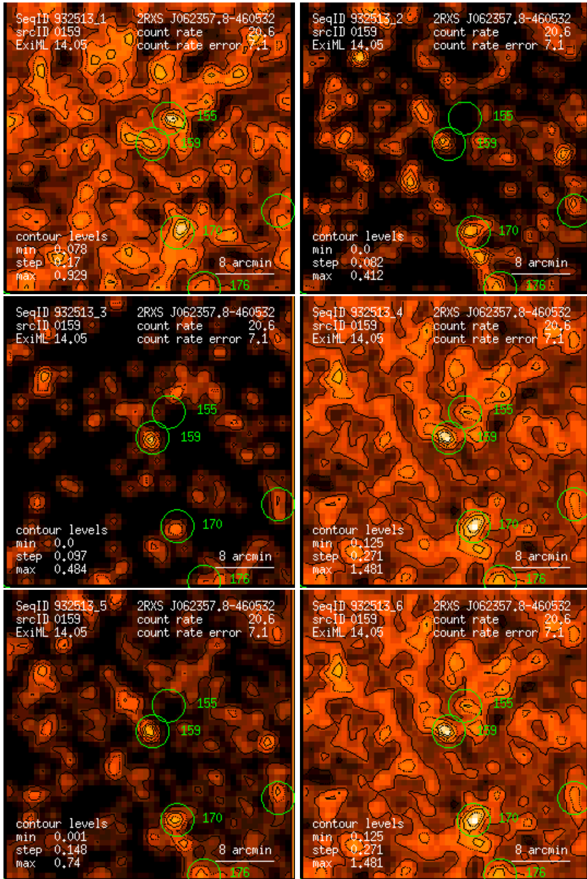
Figure 159: RASS 932513: detection 0159: band rate images, Gaussian filter: (1) PSPC channels 11 – 41, (2) 52 – 90, (3) 91 – 201, (4) 11 – 235, (5) 52 – 201, (6) 11 – 201. Broad band rates in counts/ks. Band rate contour levels in counts/ks/arcmin 2 .
