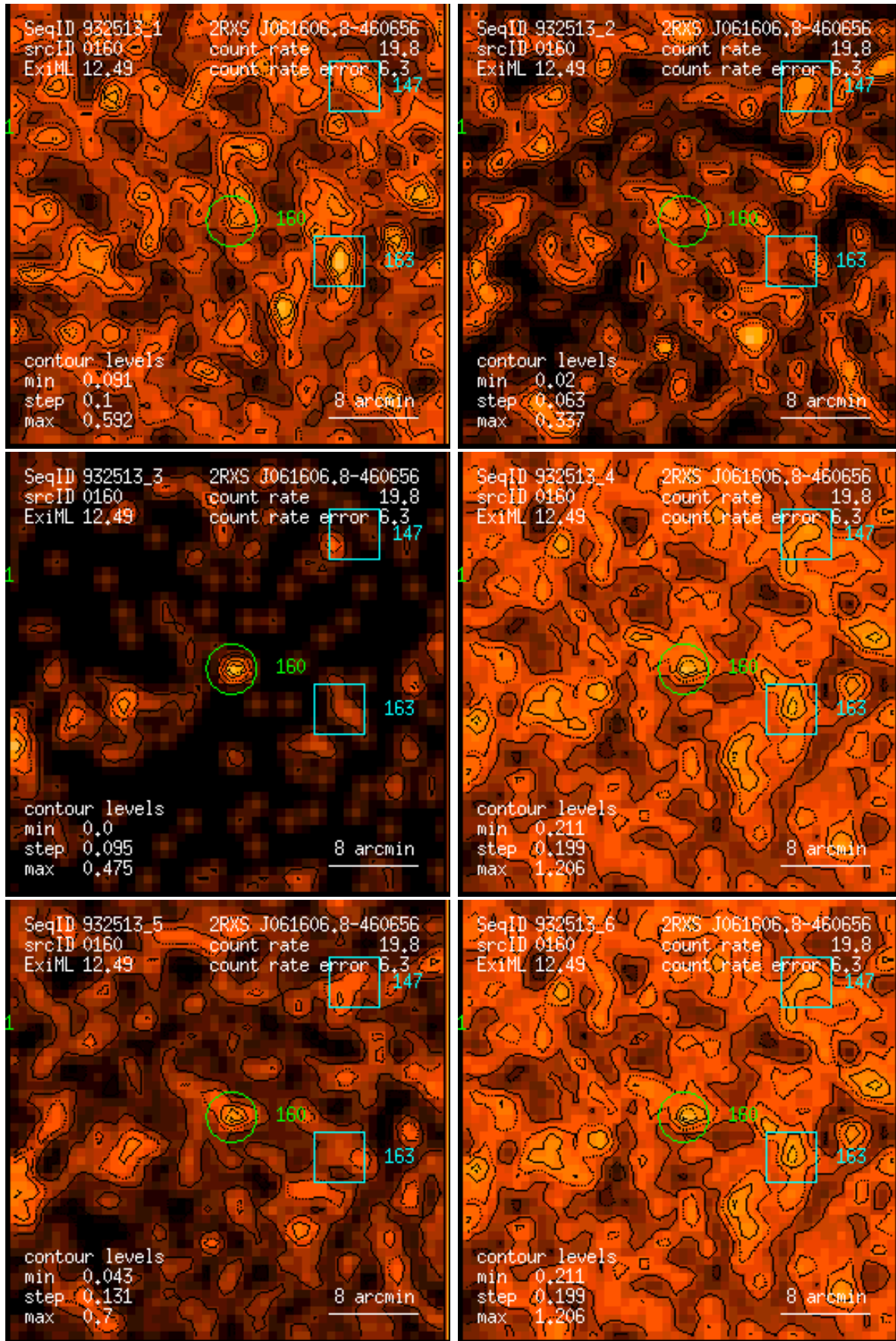
Figure 160: RASS 932513: detection 0160: band rate images, Gaussian filter: (1) PSPC channels 11 – 41, (2) 52 – 90, (3) 91 – 201, (4) 11 – 235, (5) 52 – 201, (6) 11 – 201. Broad band rates in counts/ks. Band rate contour levels in counts/ks/arcmin 2 .
