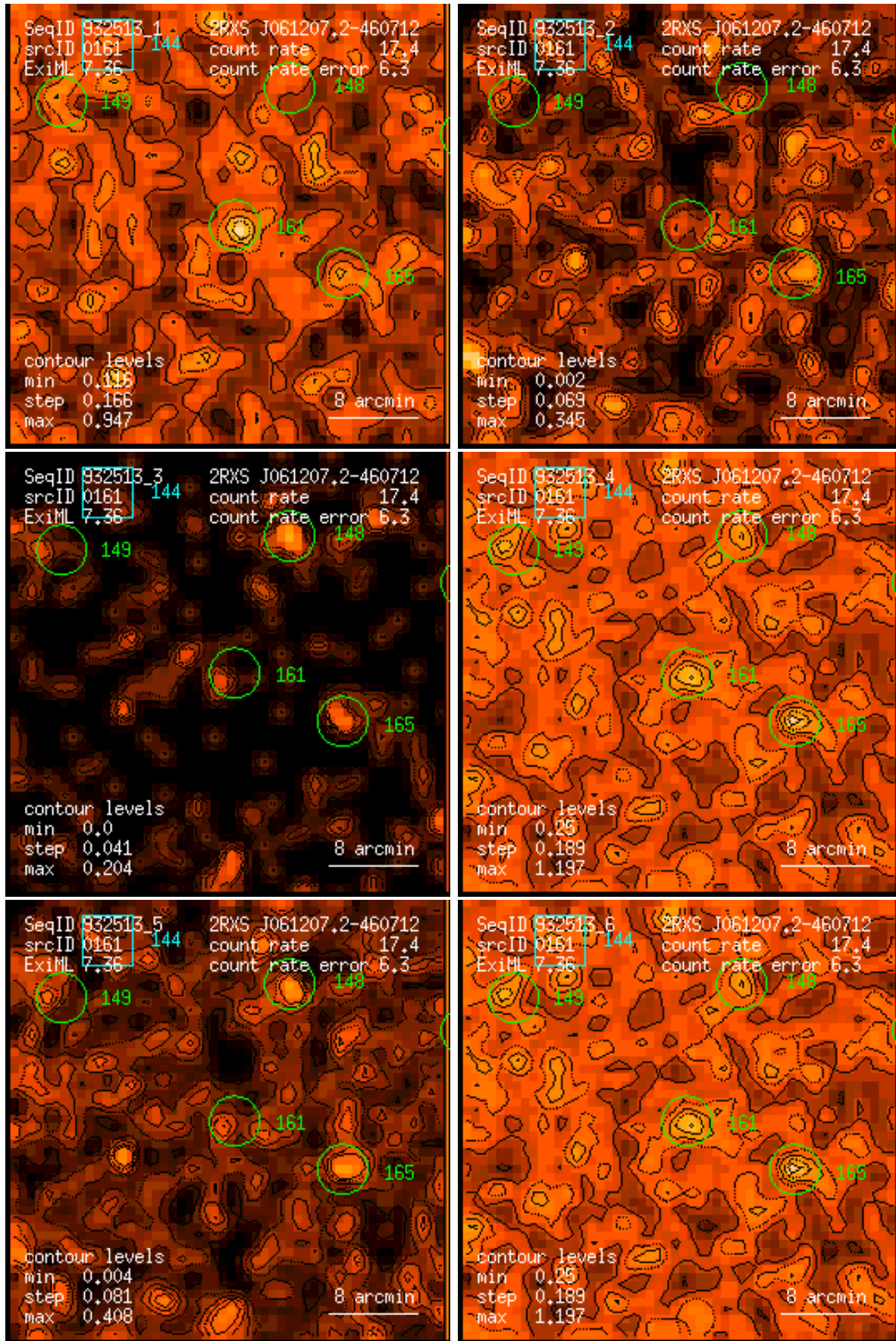
Figure 161: RASS 932513: detection 0161: band rate images, Gaussian filter: (1) PSPC channels 11 – 41, (2) 52 – 90, (3) 91 – 201, (4) 11 – 235, (5) 52 – 201, (6) 11 – 201. Broad band rates in counts/ks. Band rate contour levels in counts/ks/arcmin 2 .
