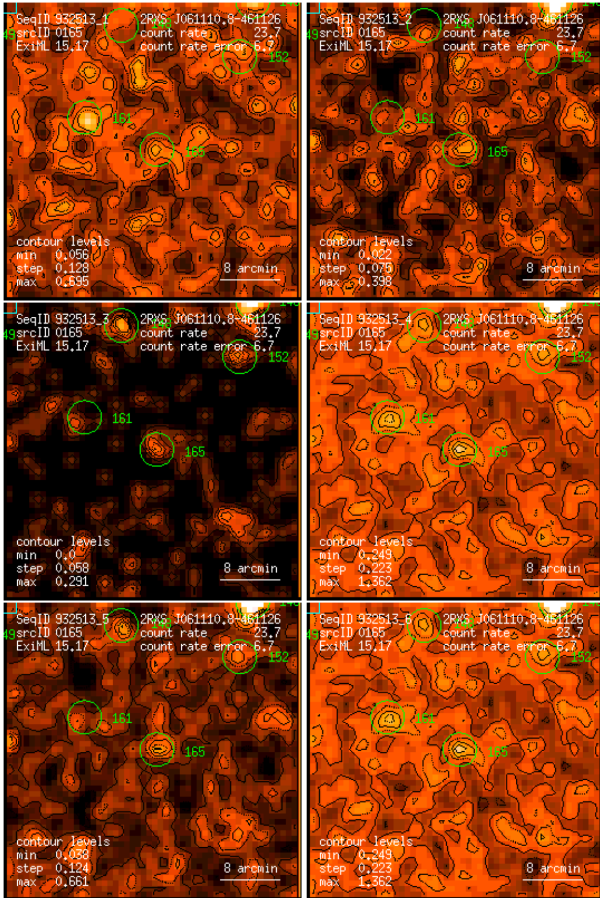
Figure 165: RASS 932513: detection 0165: band rate images, Gaussian filter: (1) PSPC channels 11 – 41, (2) 52 – 90, (3) 91 – 201, (4) 11 – 235, (5) 52 – 201, (6) 11 – 201. Broad band rates in counts/ks. Band rate contour levels in counts/ks/arcmin 2 .
