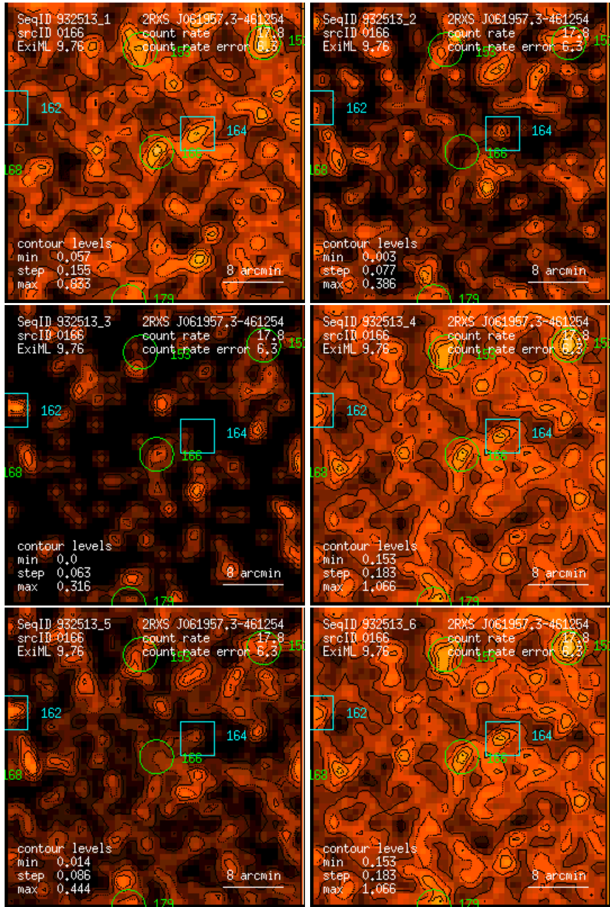
Figure 166: RASS 932513: detection 0166: band rate images, Gaussian filter: (1) PSPC channels 11 – 41, (2) 52 – 90, (3) 91 – 201, (4) 11 – 235, (5) 52 – 201, (6) 11 – 201. Broad band rates in counts/ks. Band rate contour levels in counts/ks/arcmin 2 .
