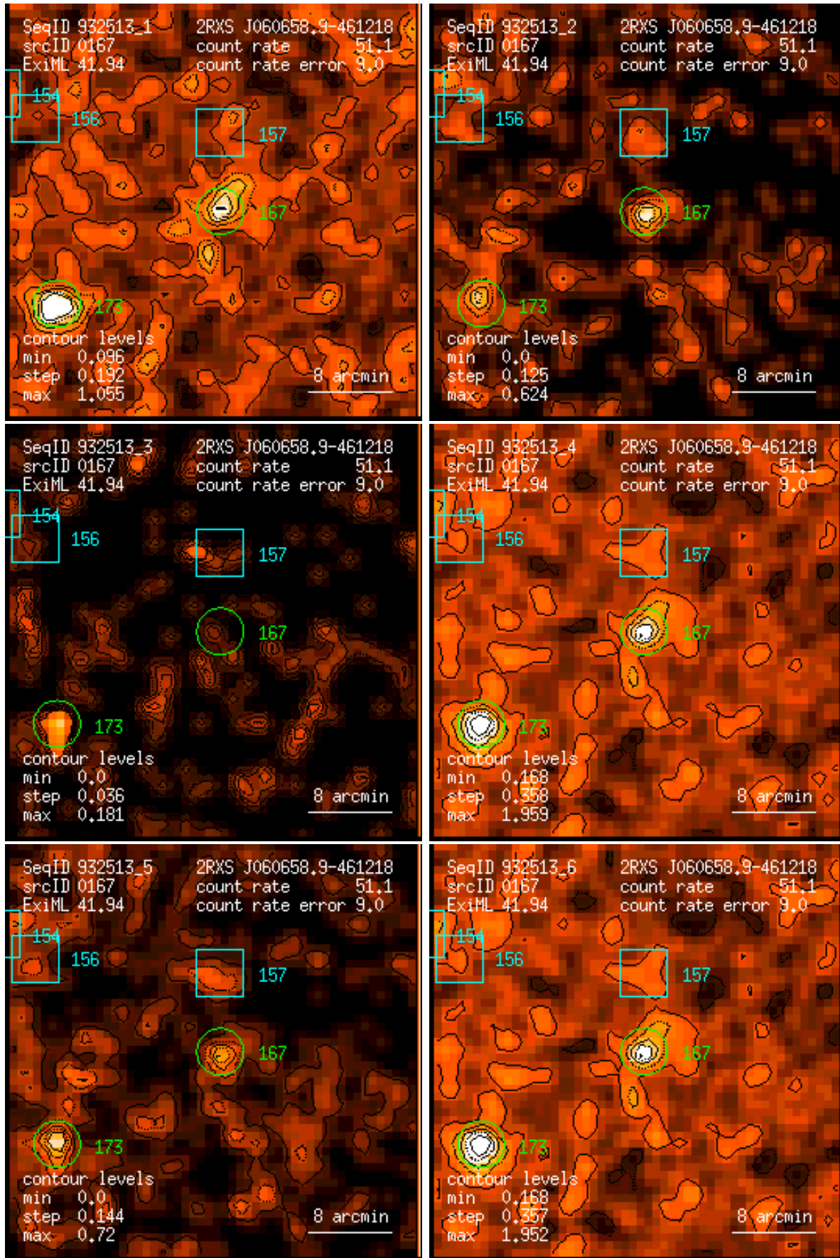
Figure 167: RASS 932513: detection 0167: band rate images, Gaussian filter: (1) PSPC channels 11 – 41, (2) 52 – 90, (3) 91 – 201, (4) 11 – 235, (5) 52 – 201, (6) 11 – 201. Broad band rates in counts/ks. Band rate contour levels in counts/ks/arcmin 2 .
