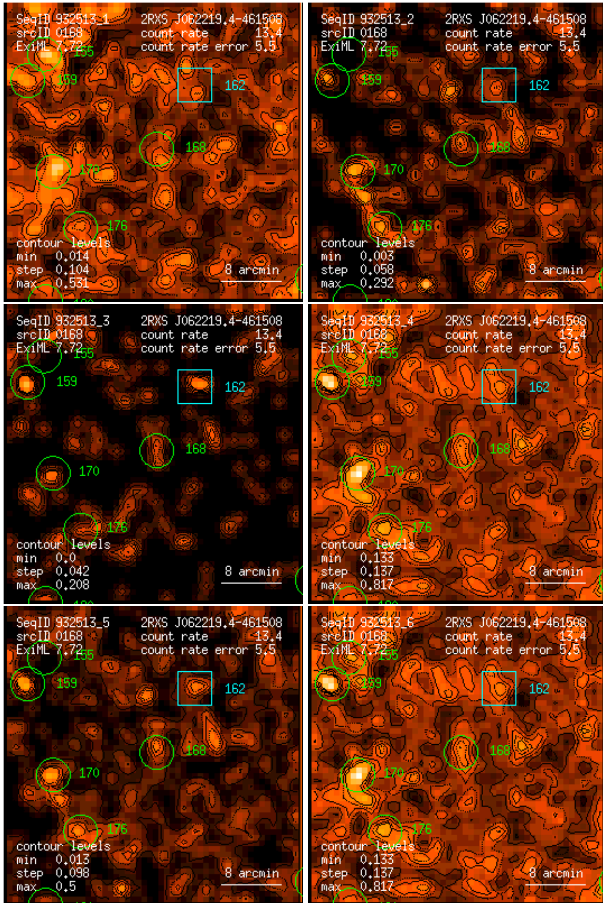
Figure 168: RASS 932513: detection 0168: band rate images, Gaussian filter: (1) PSPC channels 11 – 41, (2) 52 – 90, (3) 91 – 201, (4) 11 – 235, (5) 52 – 201, (6) 11 – 201. Broad band rates in counts/ks. Band rate contour levels in counts/ks/arcmin 2 .
