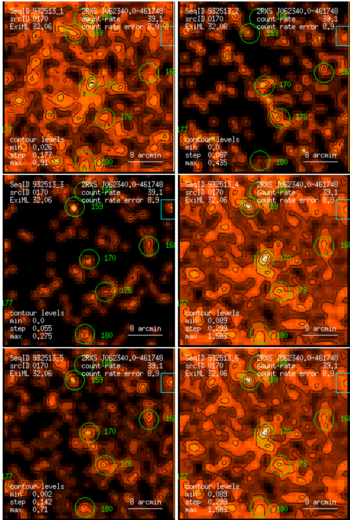
Figure 170: RASS 932513: detection 0170: band rate images, Gaussian filter: (1) PSPC channels 11 – 41, (2) 52 – 90, (3) 91 – 201, (4) 11 – 235, (5) 52 – 201, (6) 11 – 201. Broad band rates in counts/ks. Band rate contour levels in counts/ks/arcmin 2 .
