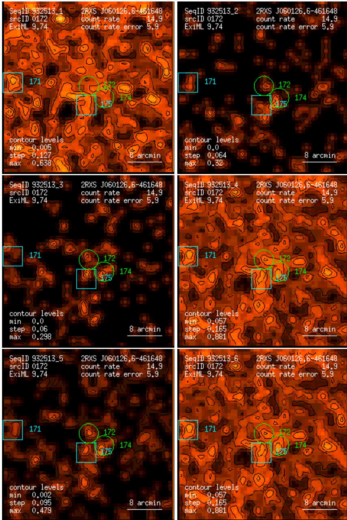
Figure 172: RASS 932513: detection 0172: band rate images, Gaussian filter: (1) PSPC channels 11 – 41, (2) 52 – 90, (3) 91 – 201, (4) 11 – 235, (5) 52 – 201, (6) 11 – 201. Broad band rates in counts/ks. Band rate contour levels in counts/ks/arcmin 2 .
