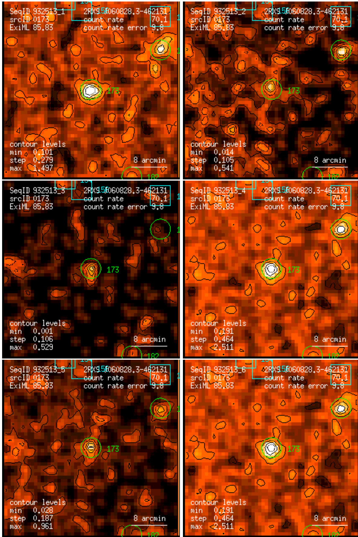
Figure 173: RASS 932513: detection 0173: band rate images, Gaussian filter: (1) PSPC channels 11 – 41, (2) 52 – 90, (3) 91 – 201, (4) 11 – 235, (5) 52 – 201, (6) 11 – 201. Broad band rates in counts/ks. Band rate contour levels in counts/ks/arcmin 2 .
