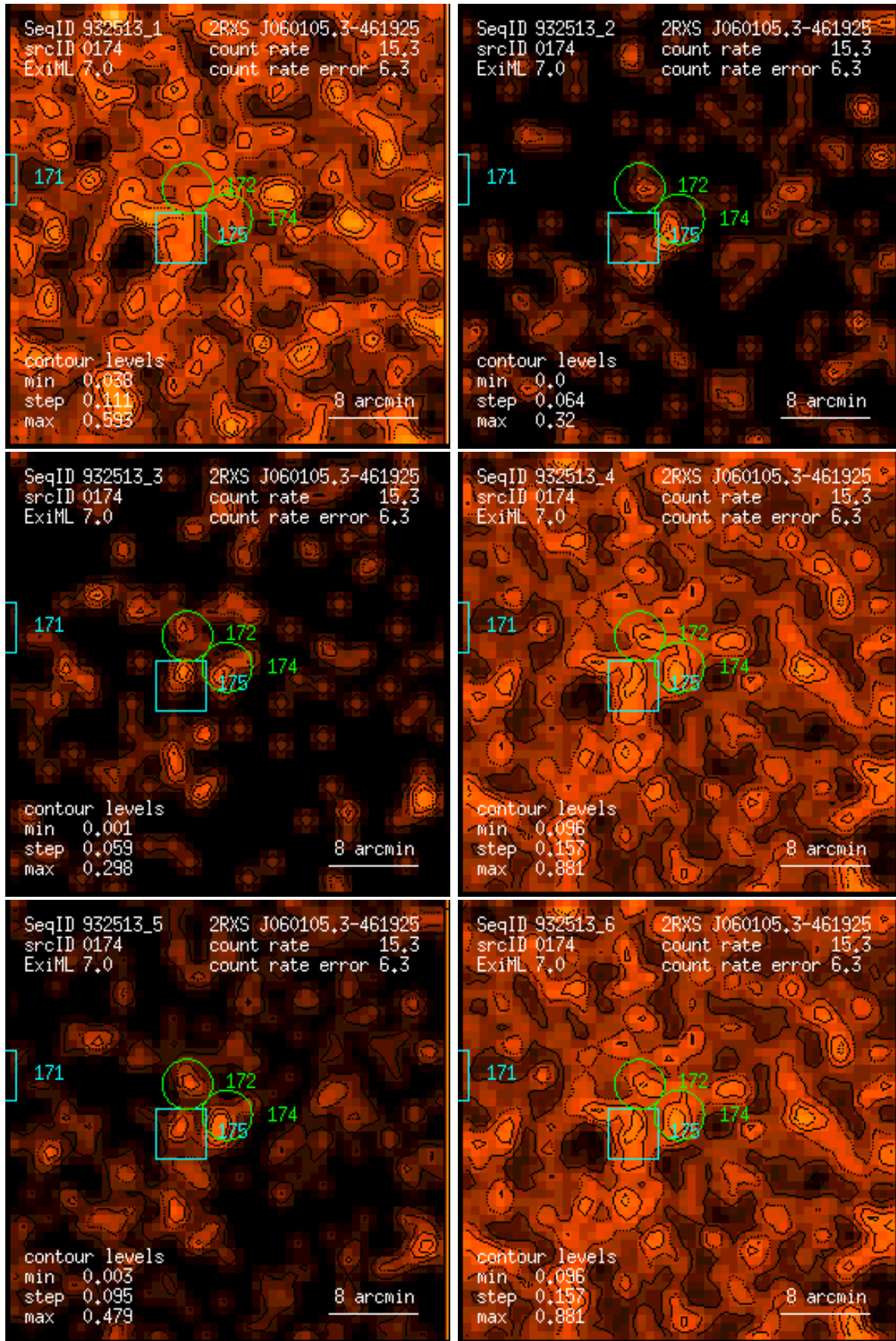
Figure 174: RASS 932513: detection 0174: band rate images, Gaussian filter: (1) PSPC channels 11 – 41, (2) 52 – 90, (3) 91 – 201, (4) 11 – 235, (5) 52 – 201, (6) 11 – 201. Broad band rates in counts/ks. Band rate contour levels in counts/ks/arcmin 2 .
