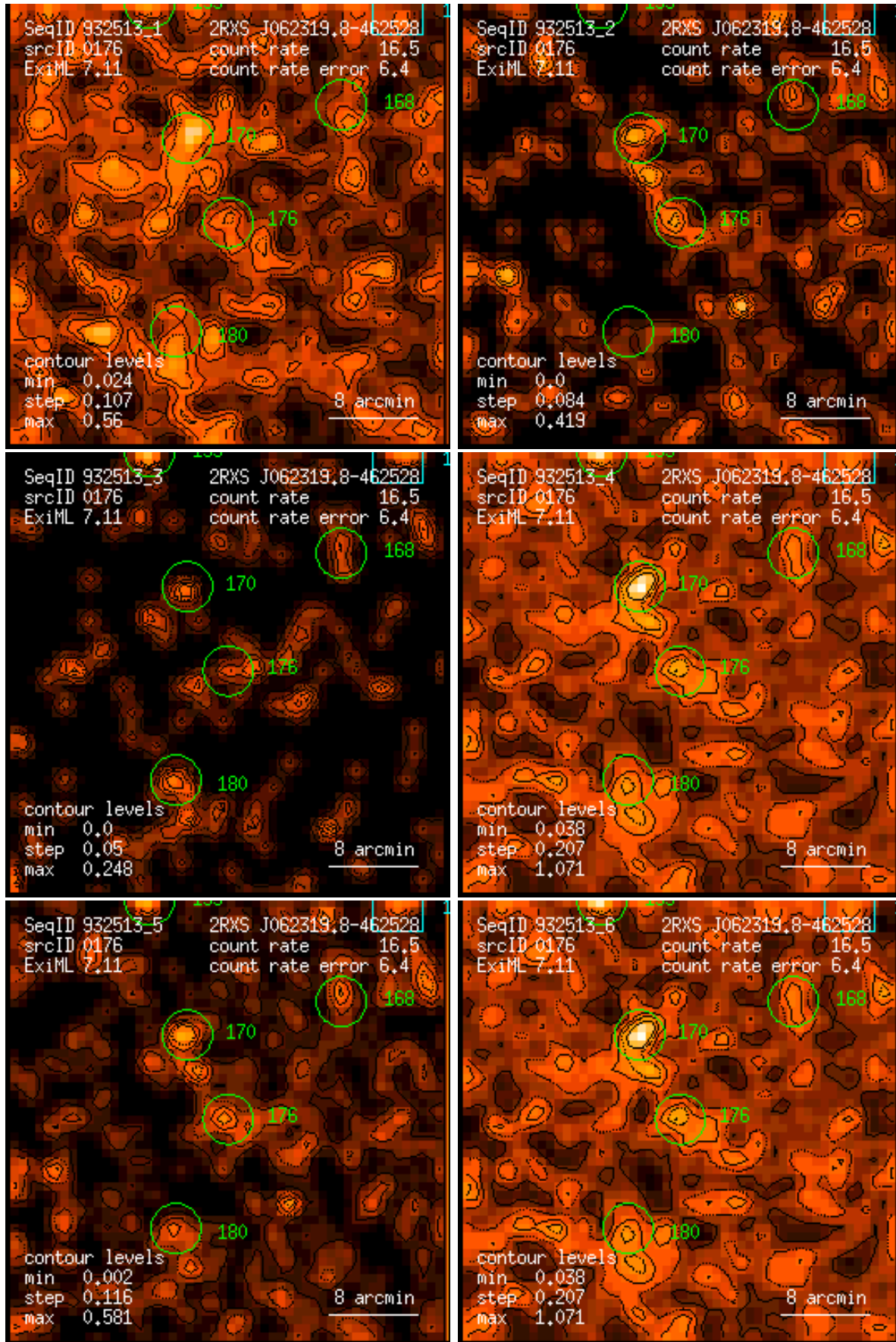
Figure 176: RASS 932513: detection 0176: band rate images, Gaussian filter: (1) PSPC channels 11 – 41, (2) 52 – 90, (3) 91 – 201, (4) 11 – 235, (5) 52 – 201, (6) 11 – 201. Broad band rates in counts/ks. Band rate contour levels in counts/ks/arcmin 2 .
