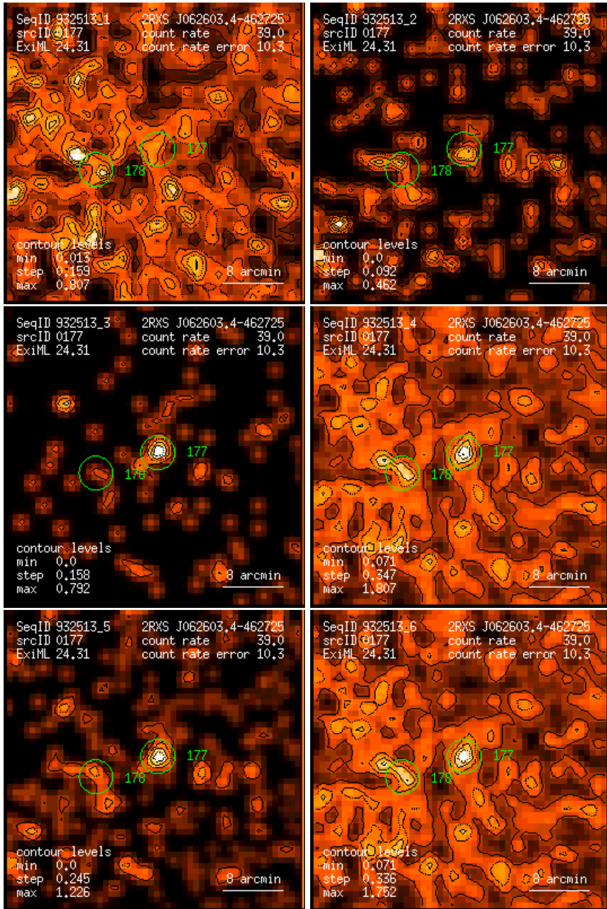
Figure 177: RASS 932513: detection 0177: band rate images, Gaussian filter: (1) PSPC channels 11 – 41, (2) 52 – 90, (3) 91 – 201, (4) 11 – 235, (5) 52 – 201, (6) 11 – 201. Broad band rates in counts/ks. Band rate contour levels in counts/ks/arcmin 2 .
