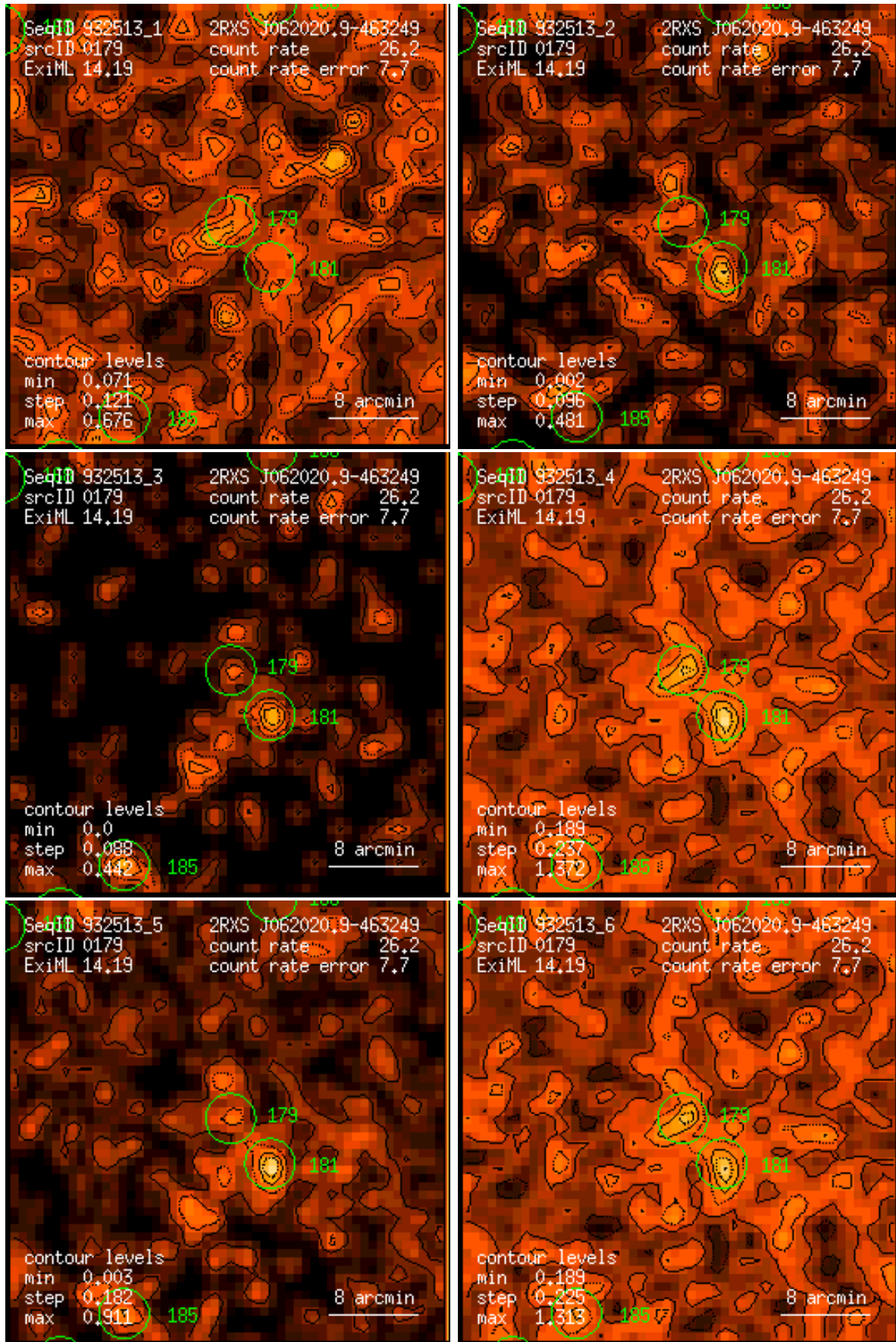
Figure 179: RASS 932513: detection 0179: band rate images, Gaussian filter: (1) PSPC channels 11 – 41, (2) 52 – 90, (3) 91 – 201, (4) 11 – 235, (5) 52 – 201, (6) 11 – 201. Broad band rates in counts/ks. Band rate contour levels in counts/ks/arcmin 2 .
