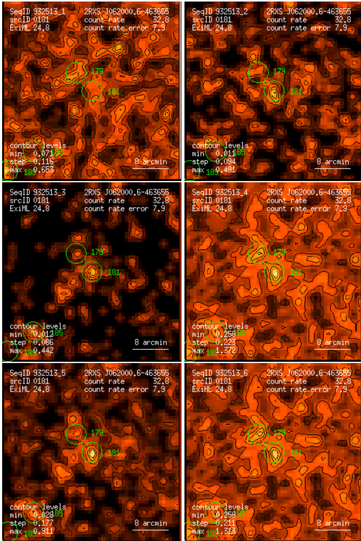
Figure 181: RASS 932513: detection 0181: band rate images, Gaussian filter: (1) PSPC channels 11 – 41, (2) 52 – 90, (3) 91 – 201, (4) 11 – 235, (5) 52 – 201, (6) 11 – 201. Broad band rates in counts/ks. Band rate contour levels in counts/ks/arcmin 2 .
