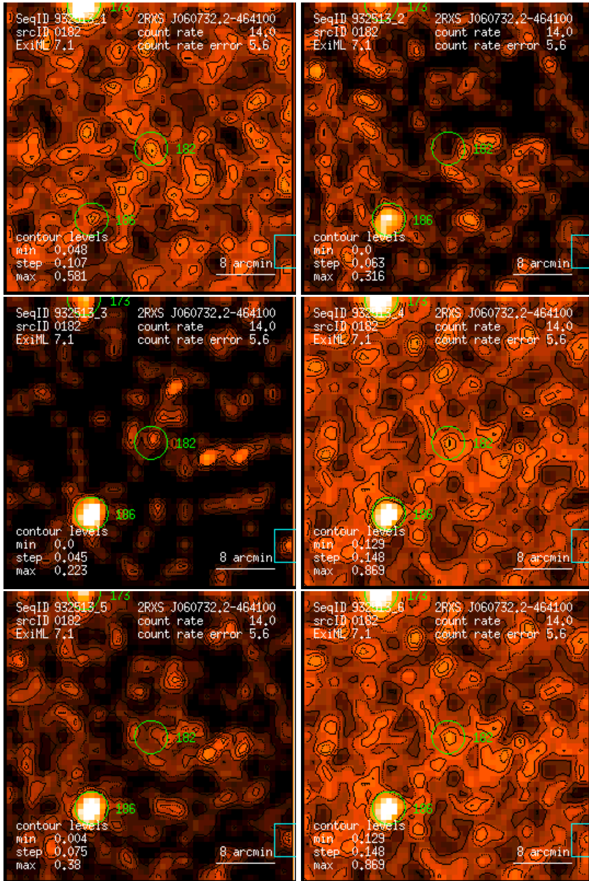
Figure 182: RASS 932513: detection 0182: band rate images, Gaussian filter: (1) PSPC channels 11 – 41, (2) 52 – 90, (3) 91 – 201, (4) 11 – 235, (5) 52 – 201, (6) 11 – 201. Broad band rates in counts/ks. Band rate contour levels in counts/ks/arcmin 2 .
