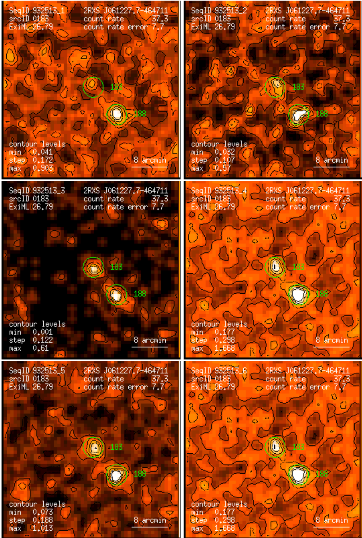
Figure 183: RASS 932513: detection 0183: band rate images, Gaussian filter: (1) PSPC channels 11 – 41, (2) 52 – 90, (3) 91 – 201, (4) 11 – 235, (5) 52 – 201, (6) 11 – 201. Broad band rates in counts/ks. Band rate contour levels in counts/ks/arcmin 2 .
