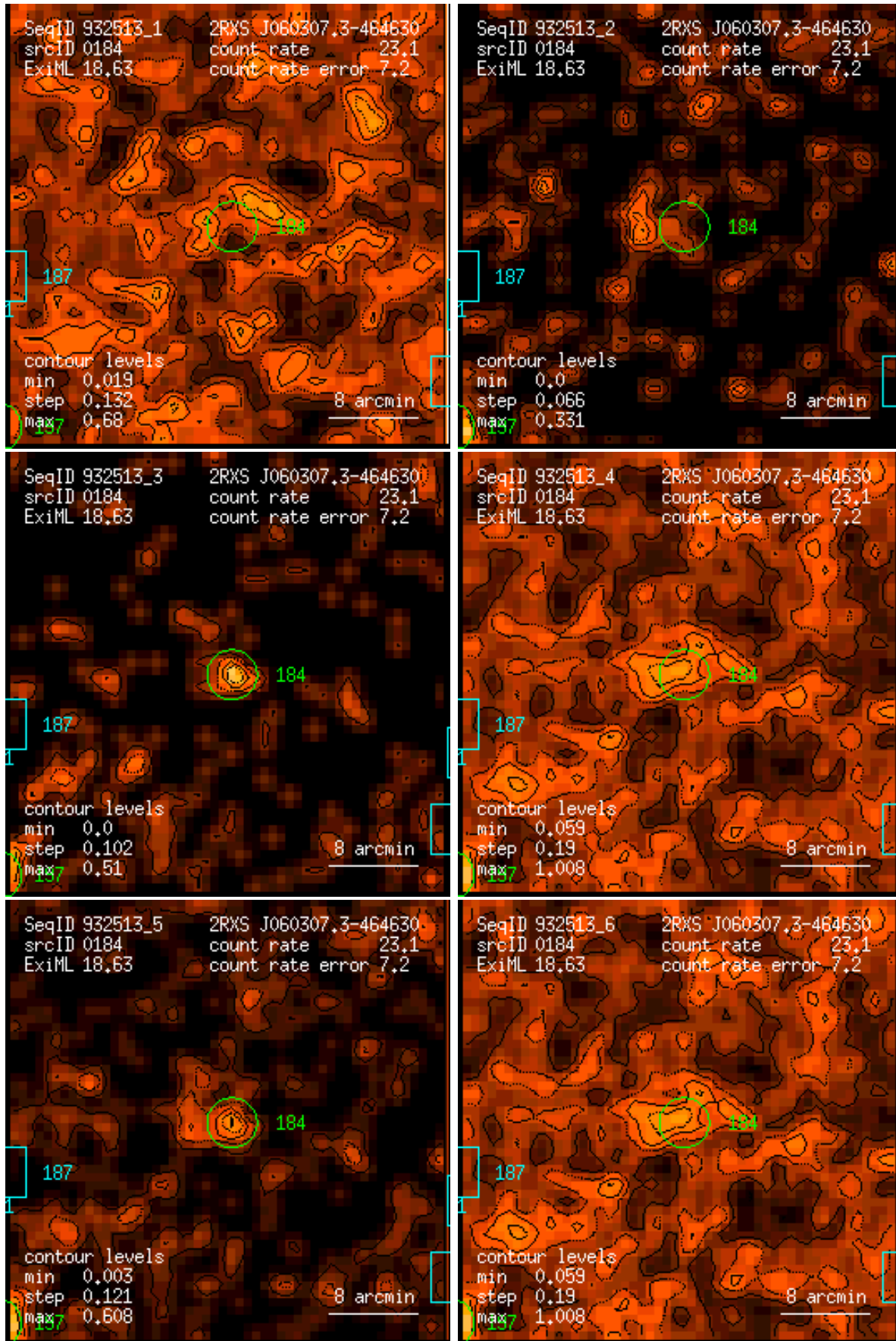
Figure 184: RASS 932513: detection 0184: band rate images, Gaussian filter: (1) PSPC channels 11 – 41, (2) 52 – 90, (3) 91 – 201, (4) 11 – 235, (5) 52 – 201, (6) 11 – 201. Broad band rates in counts/ks. Band rate contour levels in counts/ks/arcmin 2 .
