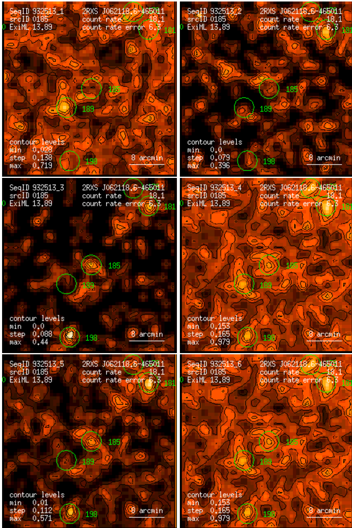
Figure 185: RASS 932513: detection 0185: band rate images, Gaussian filter: (1) PSPC channels 11 – 41, (2) 52 – 90, (3) 91 – 201, (4) 11 – 235, (5) 52 – 201, (6) 11 – 201. Broad band rates in counts/ks. Band rate contour levels in counts/ks/arcmin 2 .
