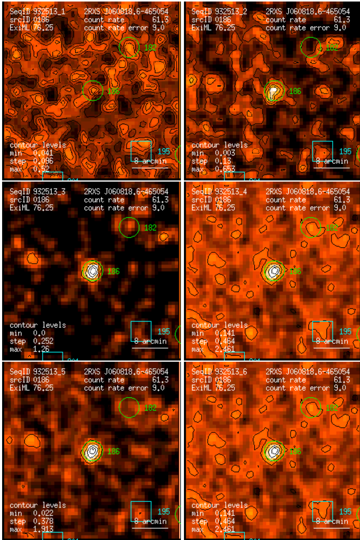
Figure 186: RASS 932513: detection 0186: band rate images, Gaussian filter: (1) PSPC channels 11 – 41, (2) 52 – 90, (3) 91 – 201, (4) 11 – 235, (5) 52 – 201, (6) 11 – 201. Broad band rates in counts/ks. Band rate contour levels in counts/ks/arcmin 2 .
