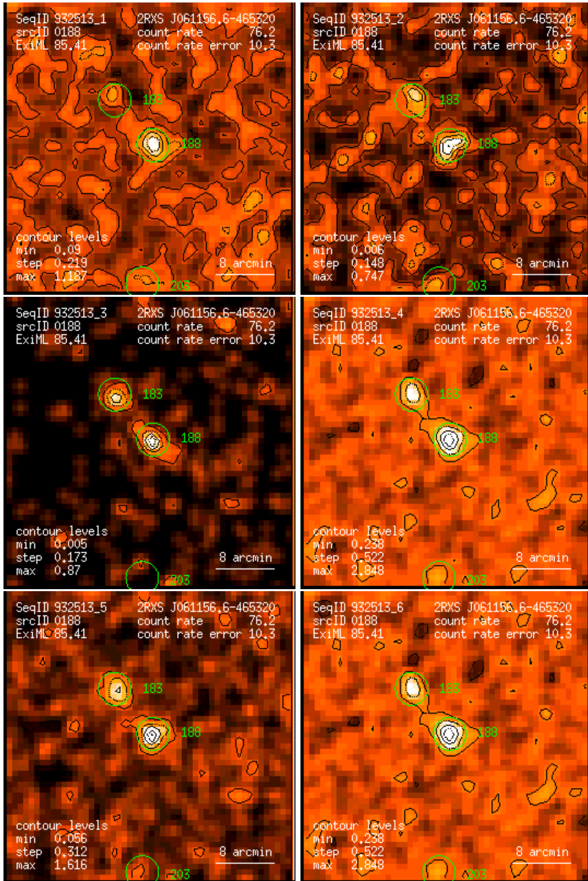
Figure 188: RASS 932513: detection 0188: band rate images, Gaussian filter: (1) PSPC channels 11 – 41, (2) 52 – 90, (3) 91 – 201, (4) 11 – 235, (5) 52 – 201, (6) 11 – 201. Broad band rates in counts/ks. Band rate contour levels in counts/ks/arcmin 2 .
