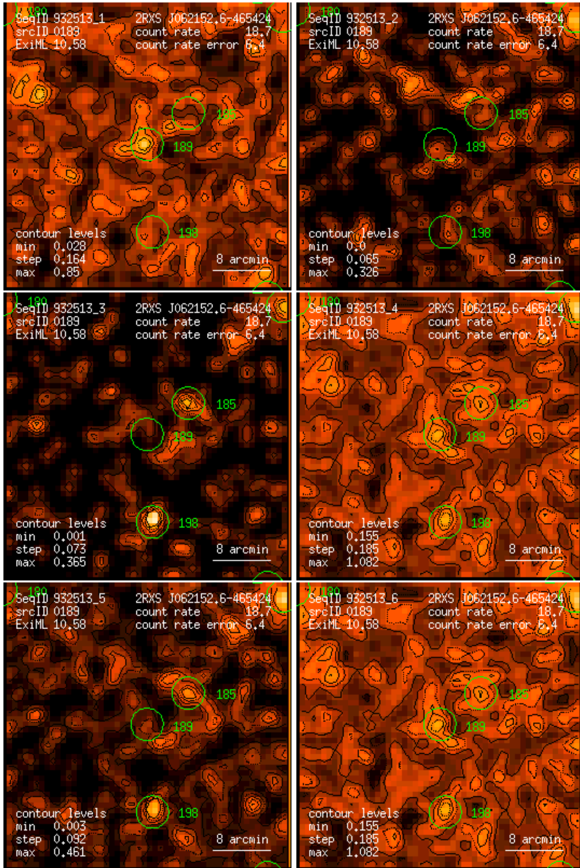
Figure 189: RASS 932513: detection 0189: band rate images, Gaussian filter: (1) PSPC channels 11 – 41, (2) 52 – 90, (3) 91 – 201, (4) 11 – 235, (5) 52 – 201, (6) 11 – 201. Broad band rates in counts/ks. Band rate contour levels in counts/ks/arcmin 2 .
