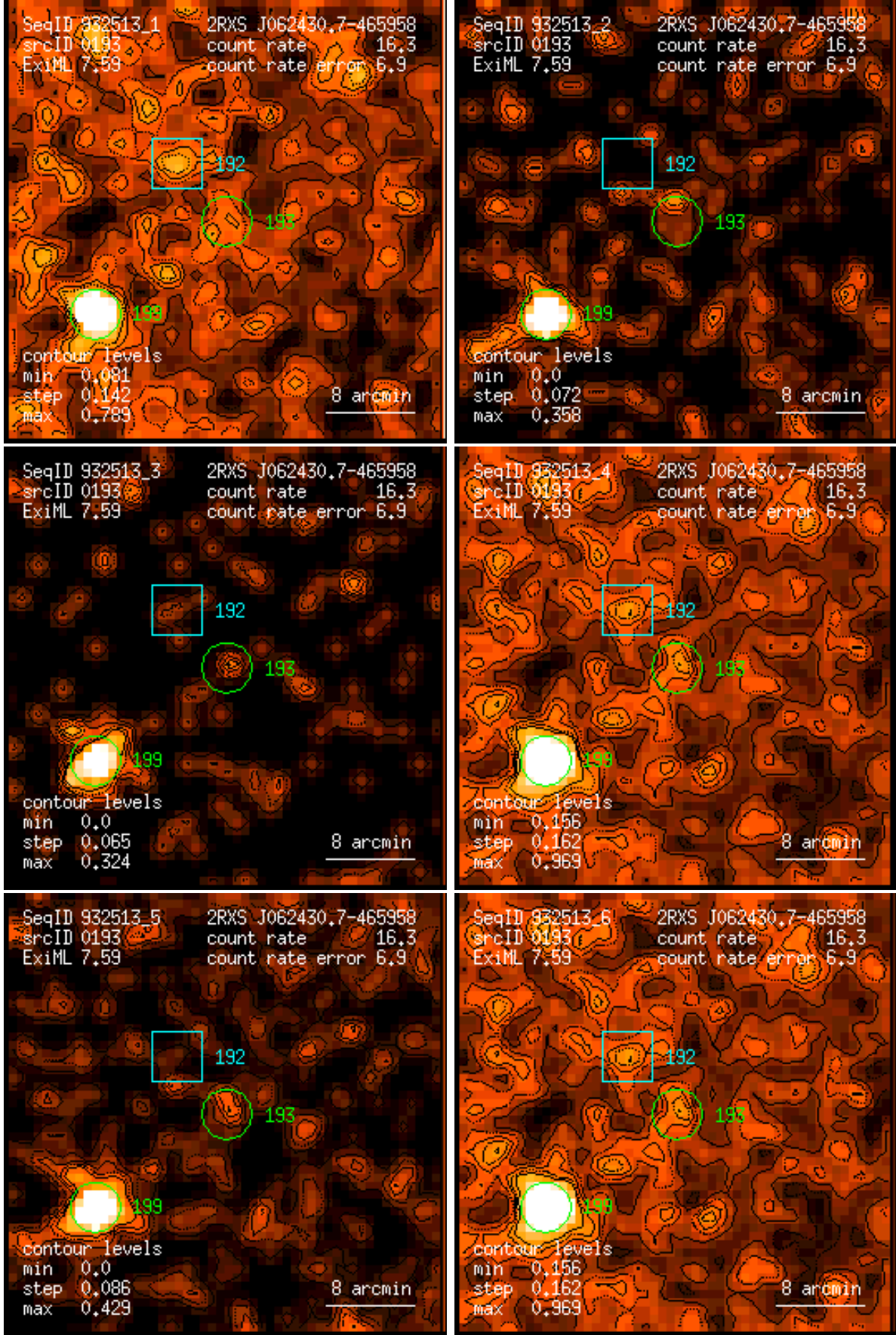
Figure 193: RASS 932513: detection 0193: band rate images, Gaussian filter: (1) PSPC channels 11 – 41, (2) 52 – 90, (3) 91 – 201, (4) 11 – 235, (5) 52 – 201, (6) 11 – 201. Broad band rates in counts/ks. Band rate contour levels in counts/ks/arcmin 2 .
