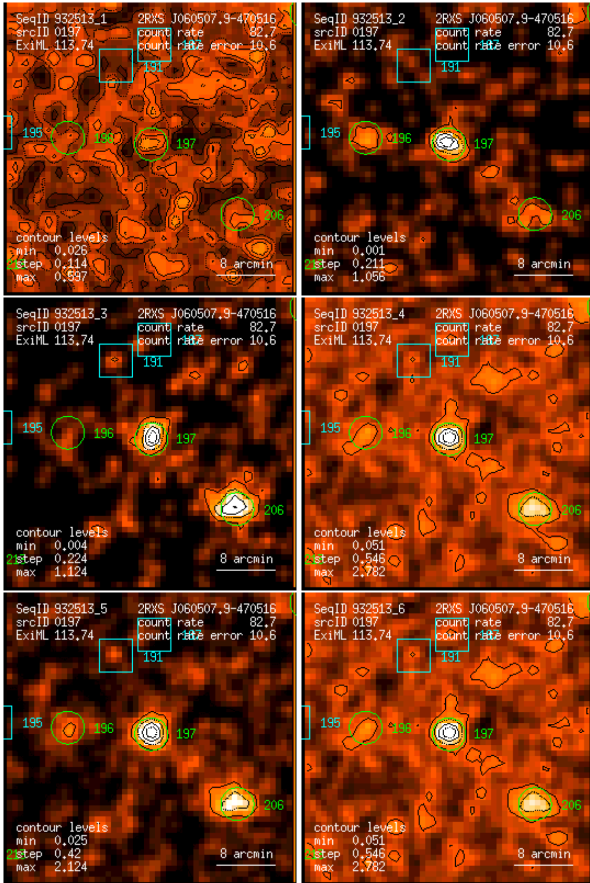
Figure 197: RASS 932513: detection 0197: band rate images, Gaussian filter: (1) PSPC channels 11 – 41, (2) 52 – 90, (3) 91 – 201, (4) 11 – 235, (5) 52 – 201, (6) 11 – 201. Broad band rates in counts/ks. Band rate contour levels in counts/ks/arcmin 2 .
