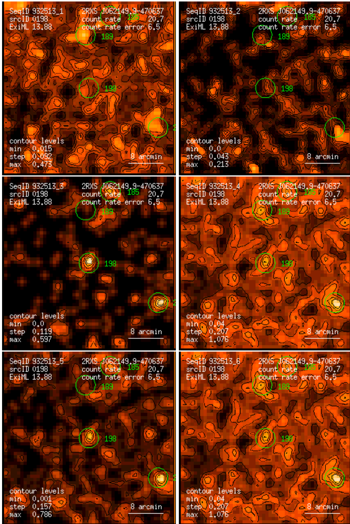
Figure 198: RASS 932513: detection 0198: band rate images, Gaussian filter: (1) PSPC channels 11 – 41, (2) 52 – 90, (3) 91 – 201, (4) 11 – 235, (5) 52 – 201, (6) 11 – 201. Broad band rates in counts/ks. Band rate contour levels in counts/ks/arcmin 2 .
