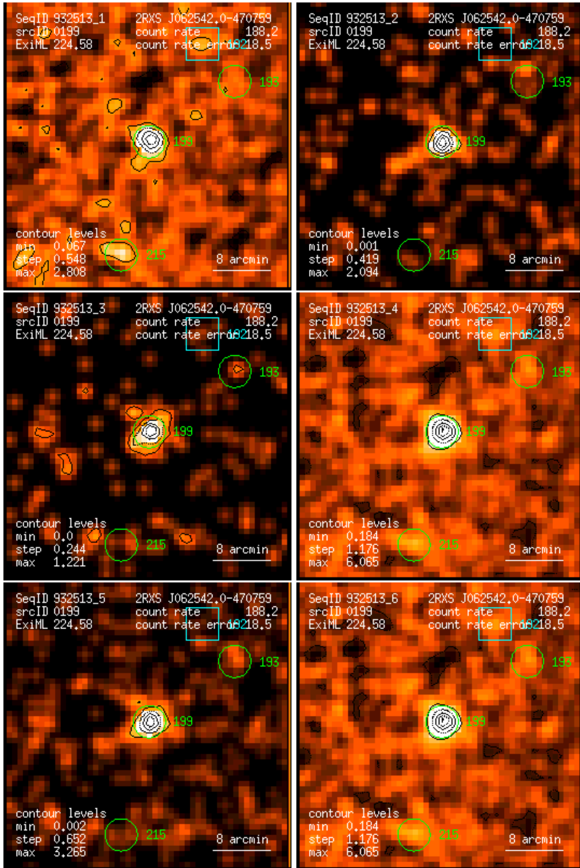
Figure 199: RASS 932513: detection 0199: band rate images, Gaussian filter: (1) PSPC channels 11 – 41, (2) 52 – 90, (3) 91 – 201, (4) 11 – 235, (5) 52 – 201, (6) 11 – 201. Broad band rates in counts/ks. Band rate contour levels in counts/ks/arcmin 2 .
