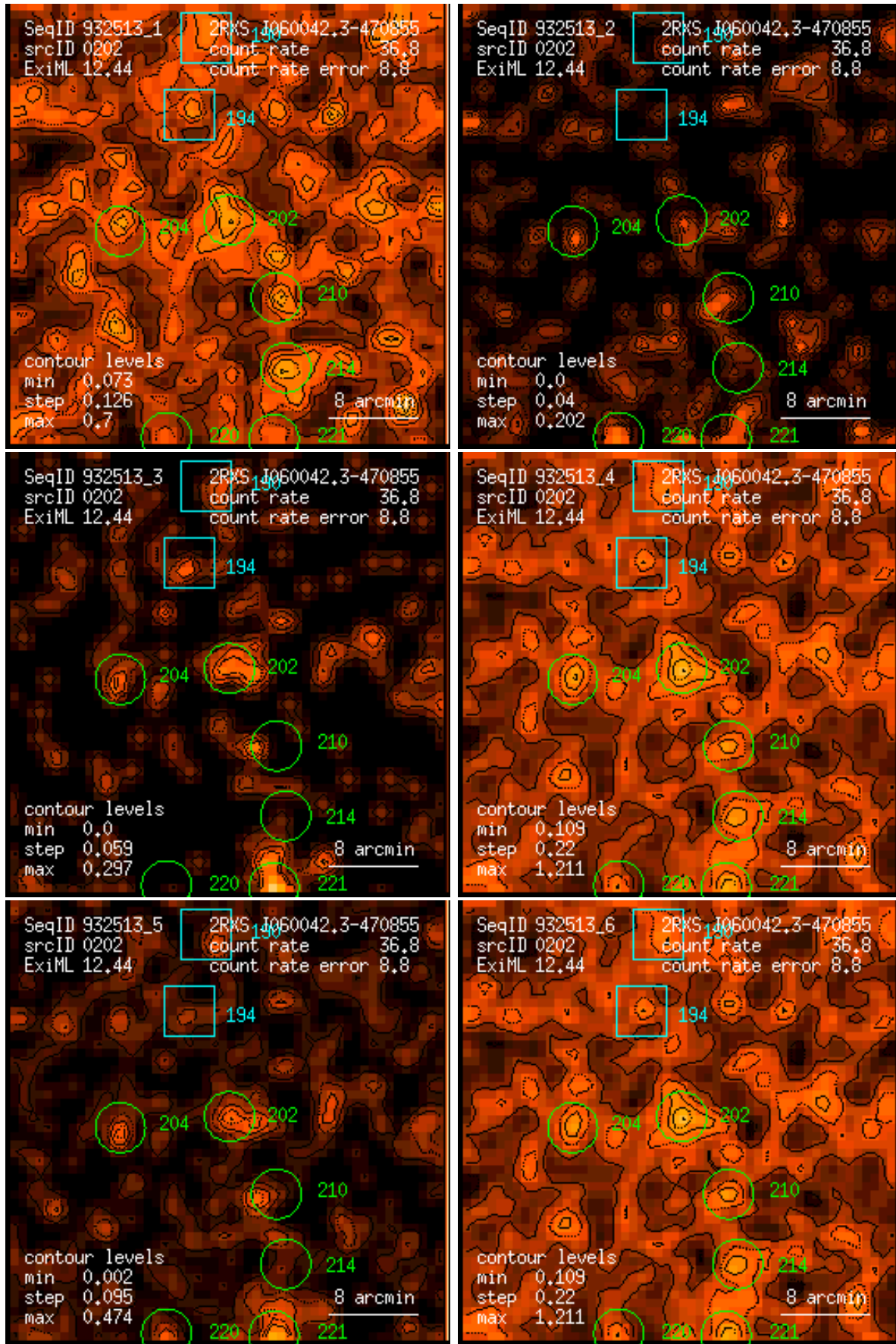
Figure 202: RASS 932513: detection 0202: band rate images, Gaussian filter: (1) PSPC channels 11 – 41, (2) 52 – 90, (3) 91 – 201, (4) 11 – 235, (5) 52 – 201, (6) 11 – 201. Broad band rates in counts/ks. Band rate contour levels in counts/ks/arcmin 2 .
