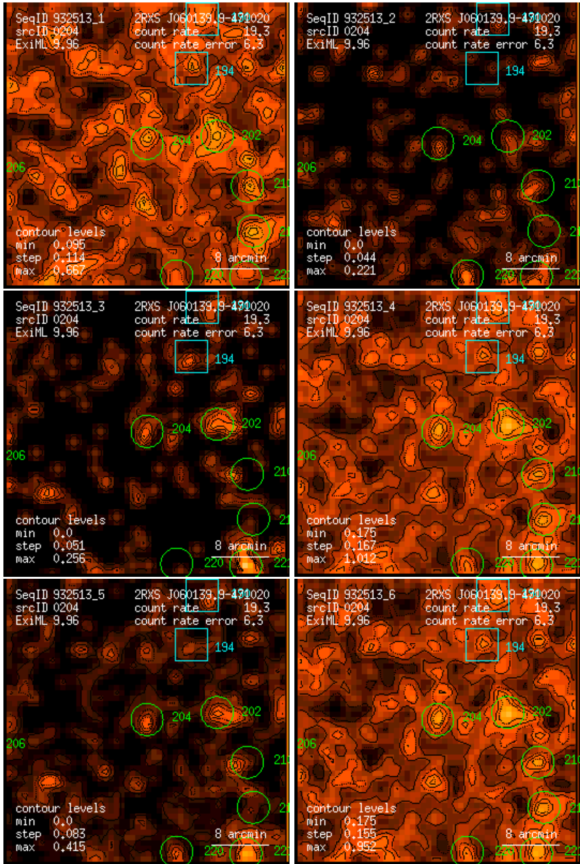
Figure 204: RASS 932513: detection 0204: band rate images, Gaussian filter: (1) PSPC channels 11 – 41, (2) 52 – 90, (3) 91 – 201, (4) 11 – 235, (5) 52 – 201, (6) 11 – 201. Broad band rates in counts/ks. Band rate contour levels in counts/ks/arcmin 2 .
