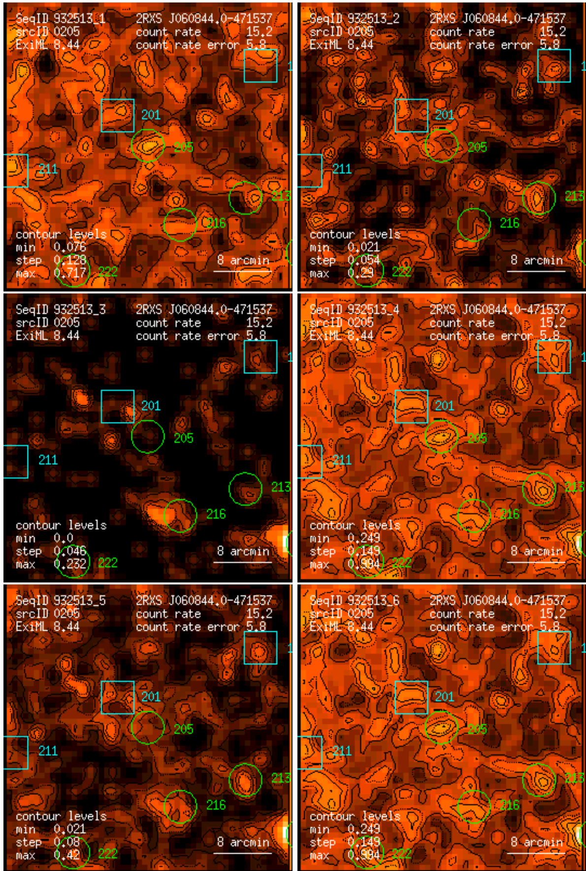
Figure 205: RASS 932513: detection 0205: band rate images, Gaussian filter: (1) PSPC channels 11 – 41, (2) 52 – 90, (3) 91 – 201, (4) 11 – 235, (5) 52 – 201, (6) 11 – 201. Broad band rates in counts/ks. Band rate contour levels in counts/ks/arcmin 2 .
