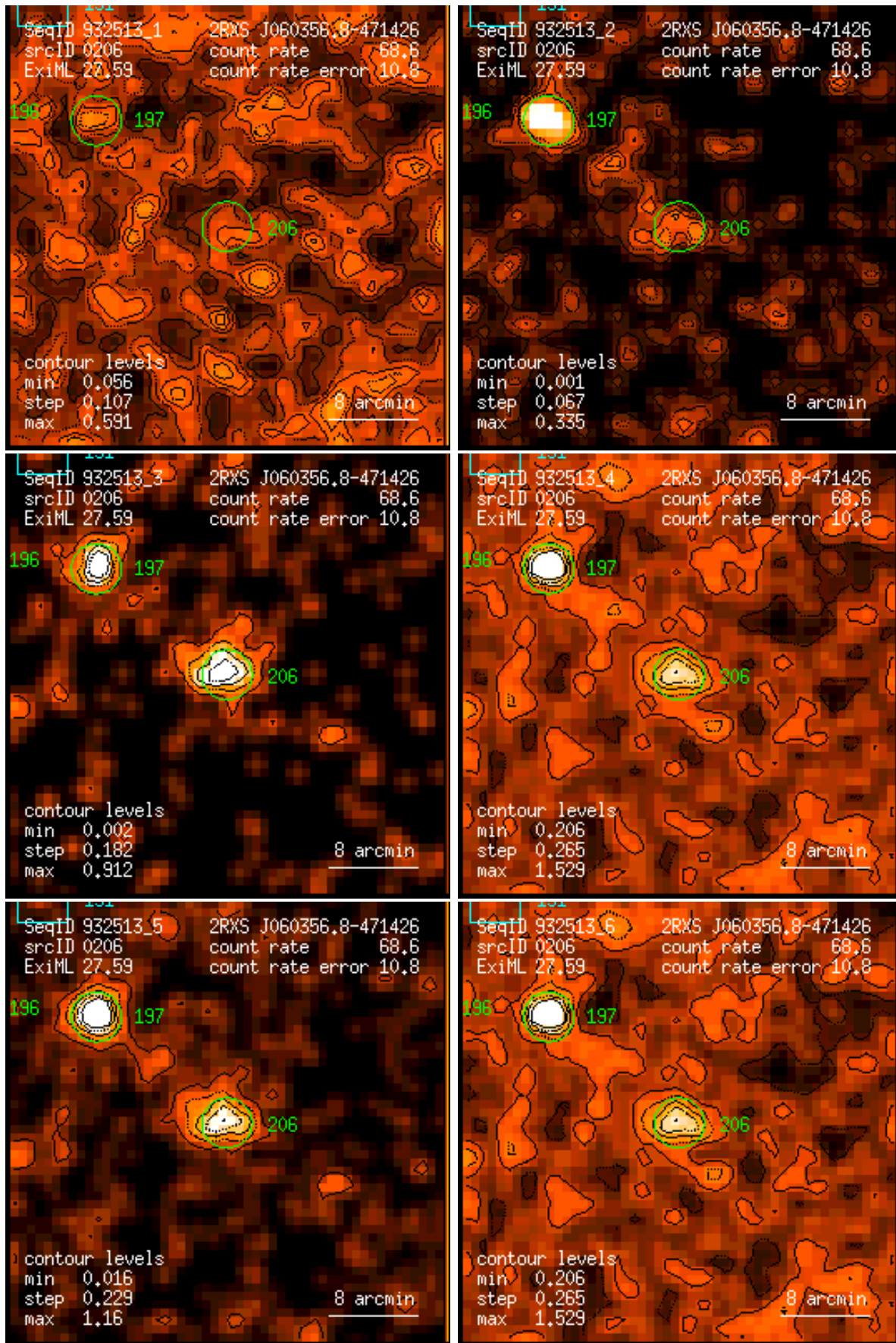
Figure 206: RASS 932513: detection 0206: band rate images, Gaussian filter: (1) PSPC channels 11 – 41, (2) 52 – 90, (3) 91 – 201, (4) 11 – 235, (5) 52 – 201, (6) 11 – 201. Broad band rates in counts/ks. Band rate contour levels in counts/ks/arcmin 2 .
