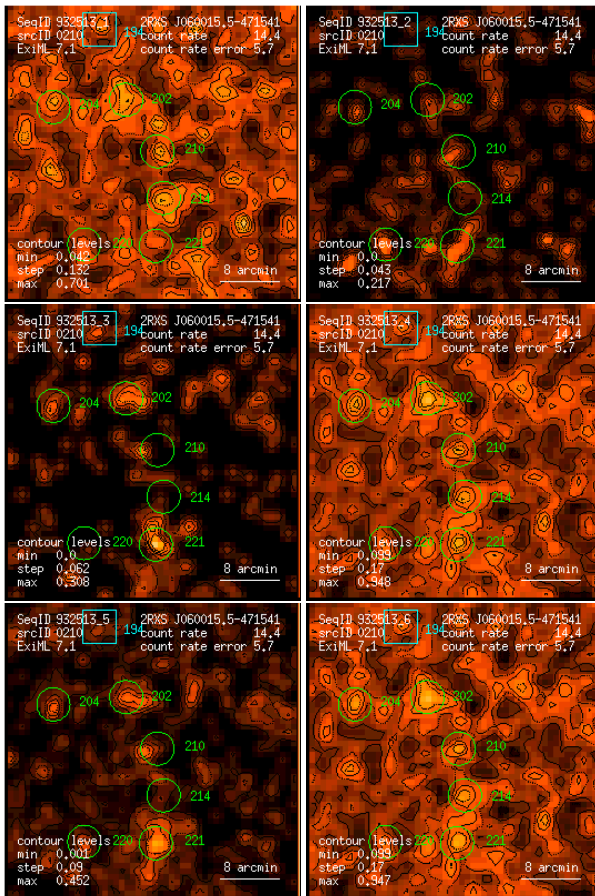
Figure 210: RASS 932513: detection 0210: band rate images, Gaussian filter: (1) PSPC channels 11 – 41, (2) 52 – 90, (3) 91 – 201, (4) 11 – 235, (5) 52 – 201, (6) 11 – 201. Broad band rates in counts/ks. Band rate contour levels in counts/ks/arcmin 2 .
