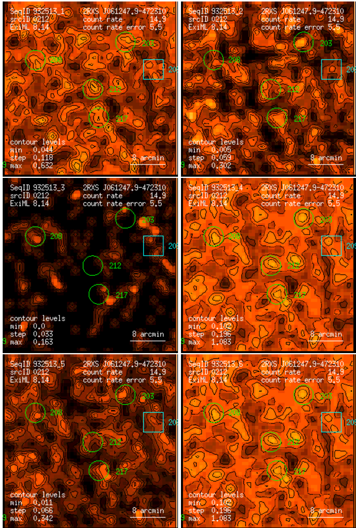
Figure 212: RASS 932513: detection 0212: band rate images, Gaussian filter: (1) PSPC channels 11 – 41, (2) 52 – 90, (3) 91 – 201, (4) 11 – 235, (5) 52 – 201, (6) 11 – 201. Broad band rates in counts/ks. Band rate contour levels in counts/ks/arcmin 2 .
