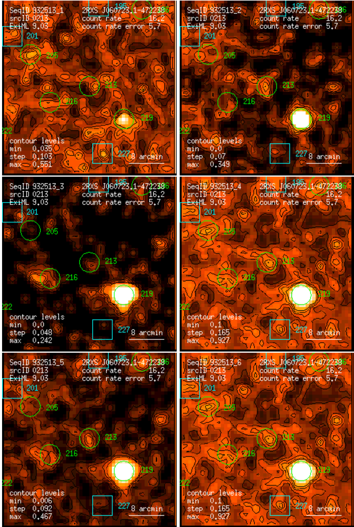
Figure 213: RASS 932513: detection 0213: band rate images, Gaussian filter: (1) PSPC channels 11 – 41, (2) 52 – 90, (3) 91 – 201, (4) 11 – 235, (5) 52 – 201, (6) 11 – 201. Broad band rates in counts/ks. Band rate contour levels in counts/ks/arcmin 2 .
