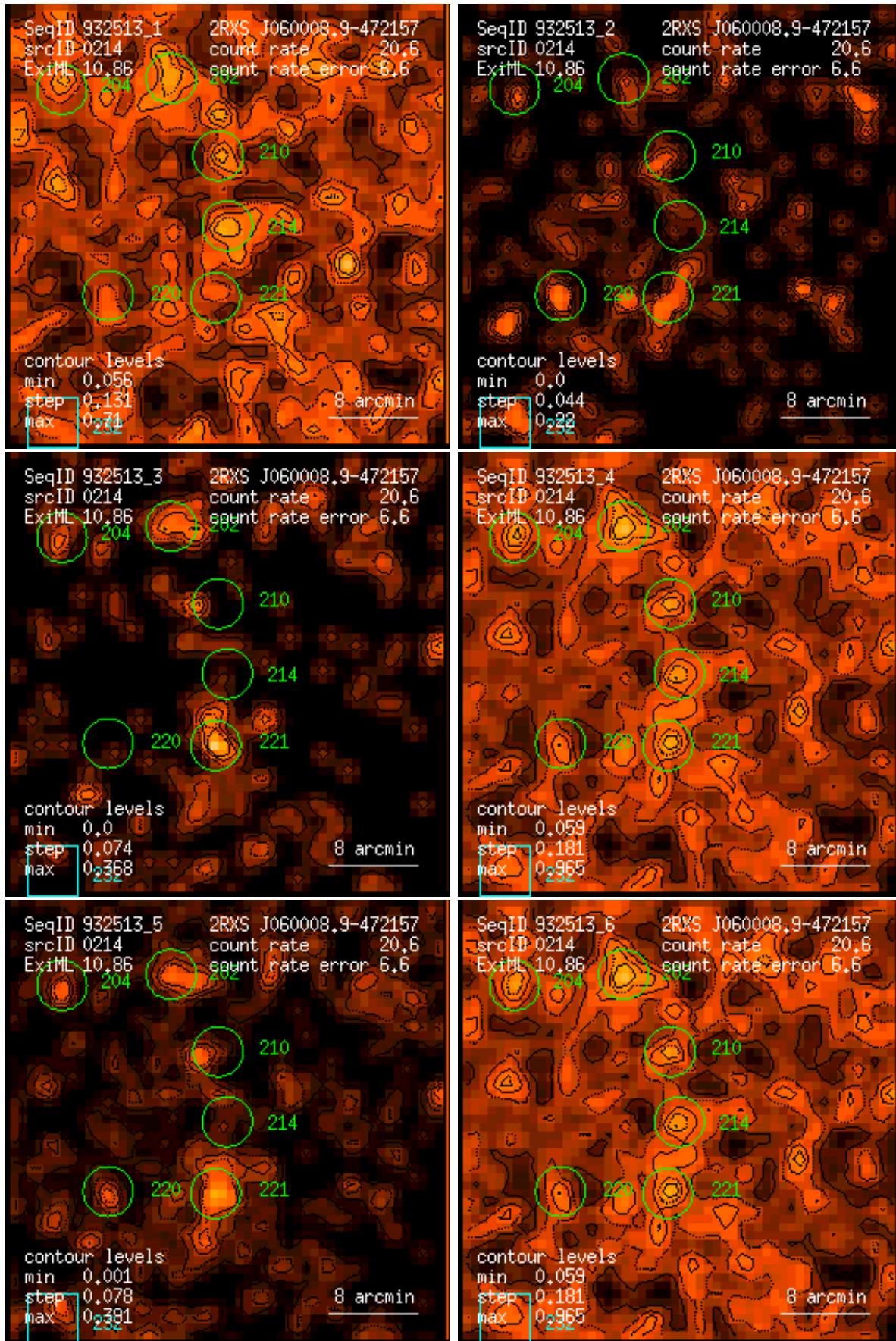
Figure 214: RASS 932513: detection 0214: band rate images, Gaussian filter: (1) PSPC channels 11 – 41, (2) 52 – 90, (3) 91 – 201, (4) 11 – 235, (5) 52 – 201, (6) 11 – 201. Broad band rates in counts/ks. Band rate contour levels in counts/ks/arcmin 2 .
