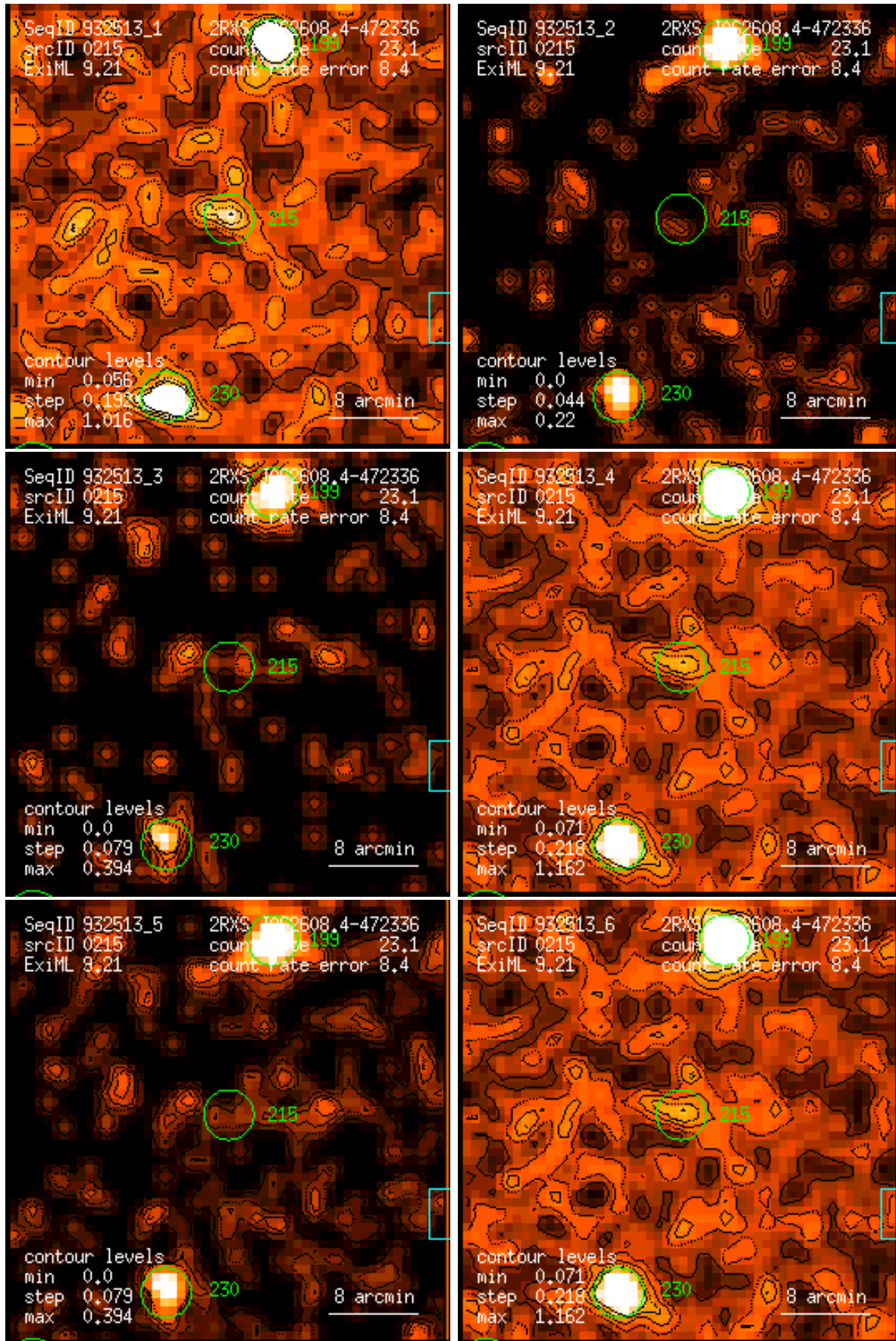
Figure 215: RASS 932513: detection 0215: band rate images, Gaussian filter: (1) PSPC channels 11 – 41, (2) 52 – 90, (3) 91 – 201, (4) 11 – 235, (5) 52 – 201, (6) 11 – 201. Broad band rates in counts/ks. Band rate contour levels in counts/ks/arcmin 2 .
