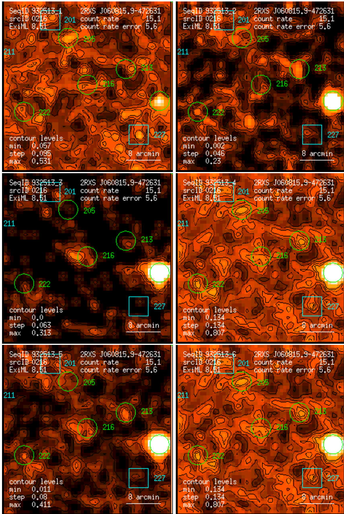
Figure 216: RASS 932513: detection 0216: band rate images, Gaussian filter: (1) PSPC channels 11 – 41, (2) 52 – 90, (3) 91 – 201, (4) 11 – 235, (5) 52 – 201, (6) 11 – 201. Broad band rates in counts/ks. Band rate contour levels in counts/ks/arcmin 2 .
