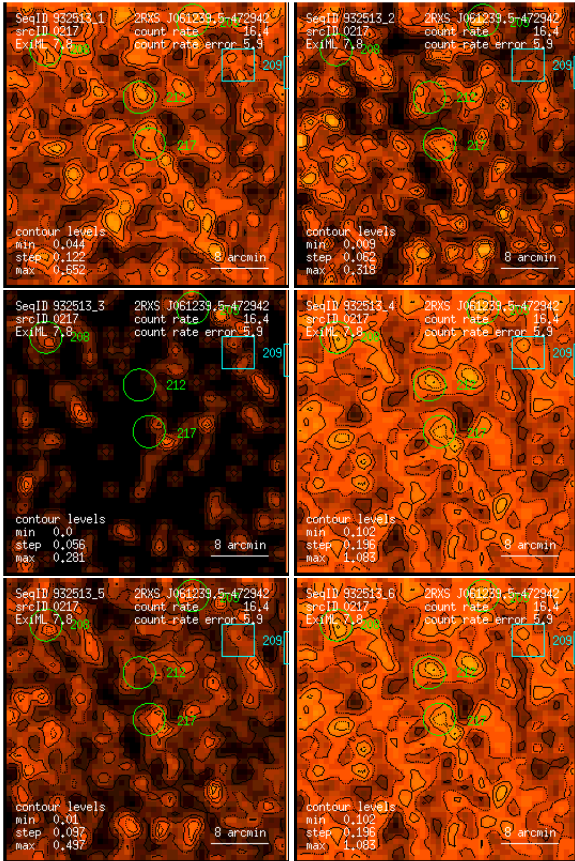
Figure 217: RASS 932513: detection 0217: band rate images, Gaussian filter: (1) PSPC channels 11 – 41, (2) 52 – 90, (3) 91 – 201, (4) 11 – 235, (5) 52 – 201, (6) 11 – 201. Broad band rates in counts/ks. Band rate contour levels in counts/ks/arcmin 2 .
