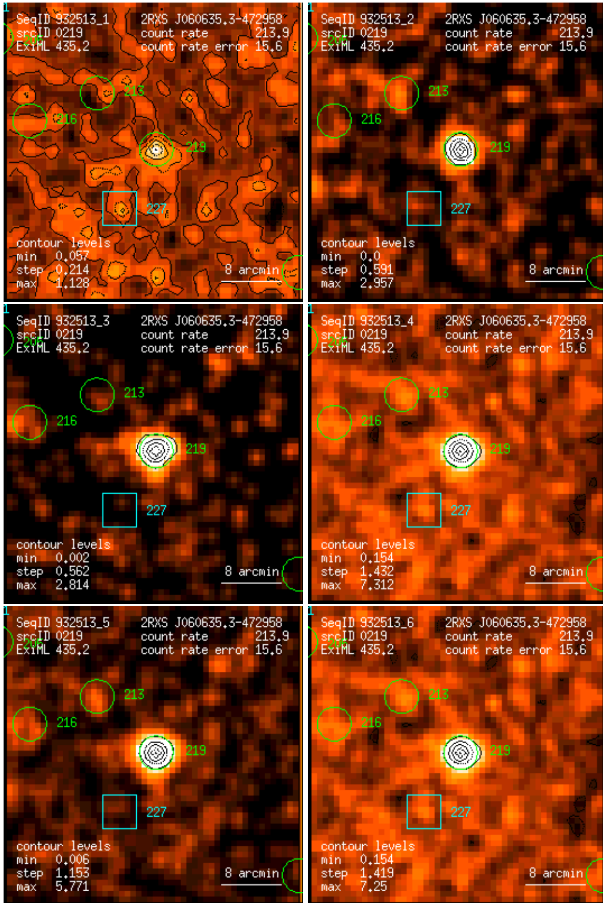
Figure 219: RASS 932513: detection 0219: band rate images, Gaussian filter: (1) PSPC channels 11 – 41, (2) 52 – 90, (3) 91 – 201, (4) 11 – 235, (5) 52 – 201, (6) 11 – 201. Broad band rates in counts/ks. Band rate contour levels in counts/ks/arcmin 2 .
