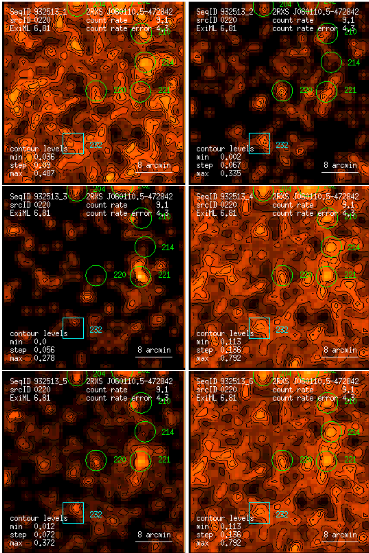
Figure 220: RASS 932513: detection 0220: band rate images, Gaussian filter: (1) PSPC channels 11 – 41, (2) 52 – 90, (3) 91 – 201, (4) 11 – 235, (5) 52 – 201, (6) 11 – 201. Broad band rates in counts/ks. Band rate contour levels in counts/ks/arcmin 2 .
