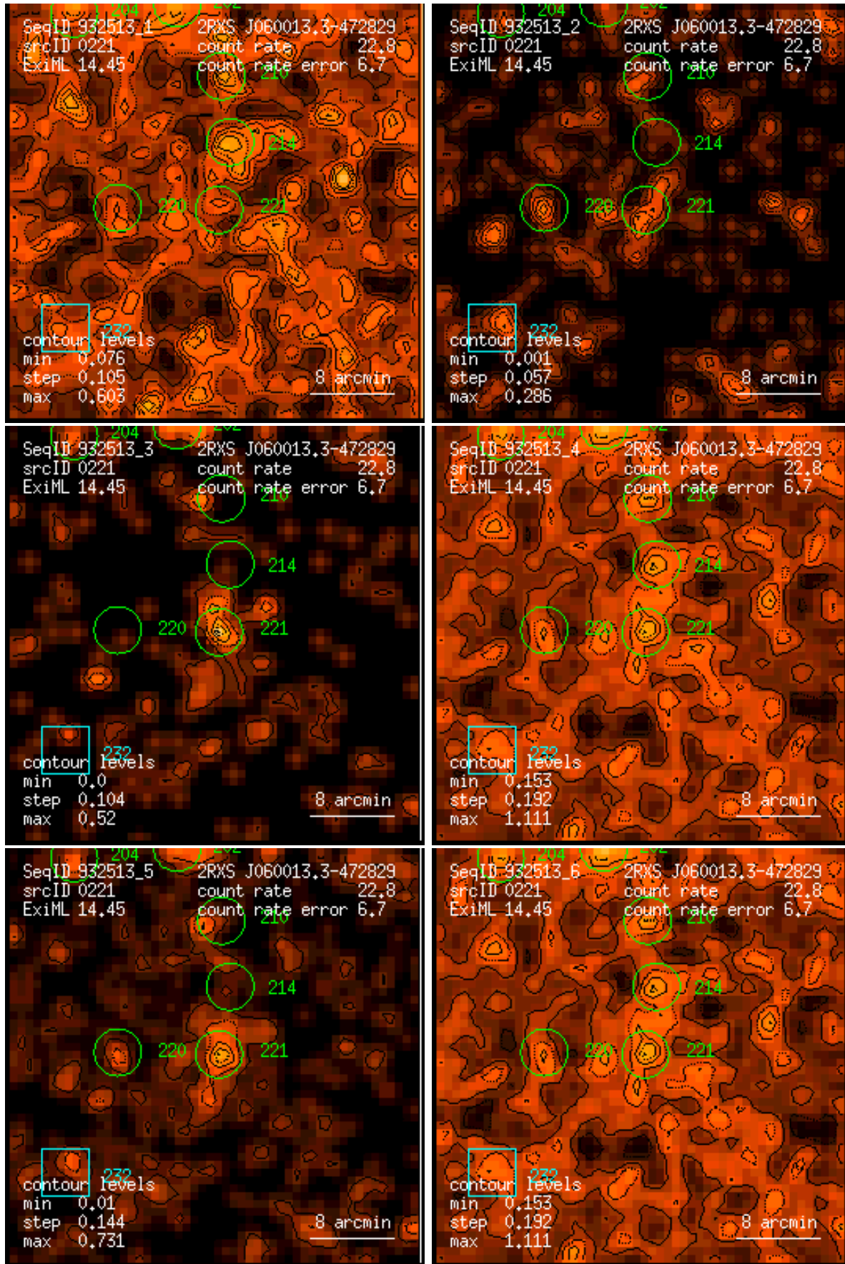
Figure 221: RASS 932513: detection 0221: band rate images, Gaussian filter: (1) PSPC channels 11 – 41, (2) 52 – 90, (3) 91 – 201, (4) 11 – 235, (5) 52 – 201, (6) 11 – 201. Broad band rates in counts/ks. Band rate contour levels in counts/ks/arcmin 2 .
