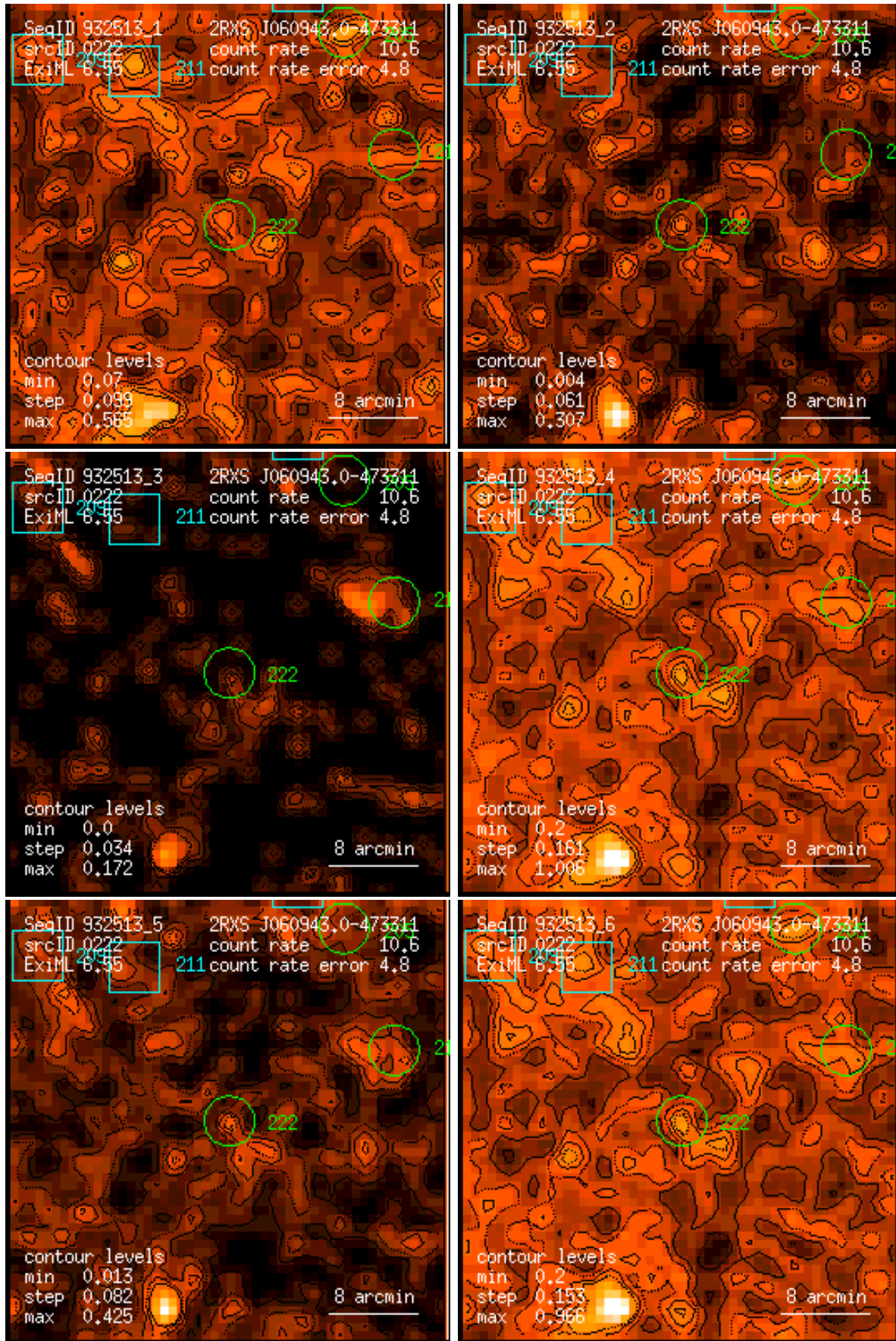
Figure 222: RASS 932513: detection 0222: band rate images, Gaussian filter: (1) PSPC channels 11 – 41, (2) 52 – 90, (3) 91 – 201, (4) 11 – 235, (5) 52 – 201, (6) 11 – 201. Broad band rates in counts/ks. Band rate contour levels in counts/ks/arcmin 2 .
