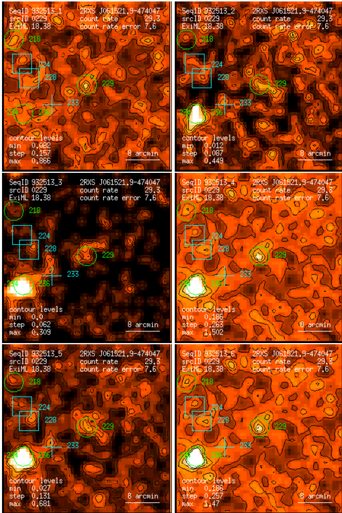
Figure 229: RASS 932513: detection 0229: band rate images, Gaussian filter: (1) PSPC channels 11 – 41, (2) 52 – 90, (3) 91 – 201, (4) 11 – 235, (5) 52 – 201, (6) 11 – 201. Broad band rates in counts/ks. Band rate contour levels in counts/ks/arcmin 2 .
