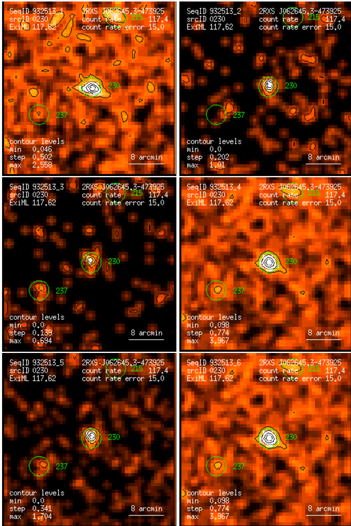
Figure 230: RASS 932513: detection 0230: band rate images, Gaussian filter: (1) PSPC channels 11 – 41, (2) 52 – 90, (3) 91 – 201, (4) 11 – 235, (5) 52 – 201, (6) 11 – 201. Broad band rates in counts/ks. Band rate contour levels in counts/ks/arcmin 2 .
