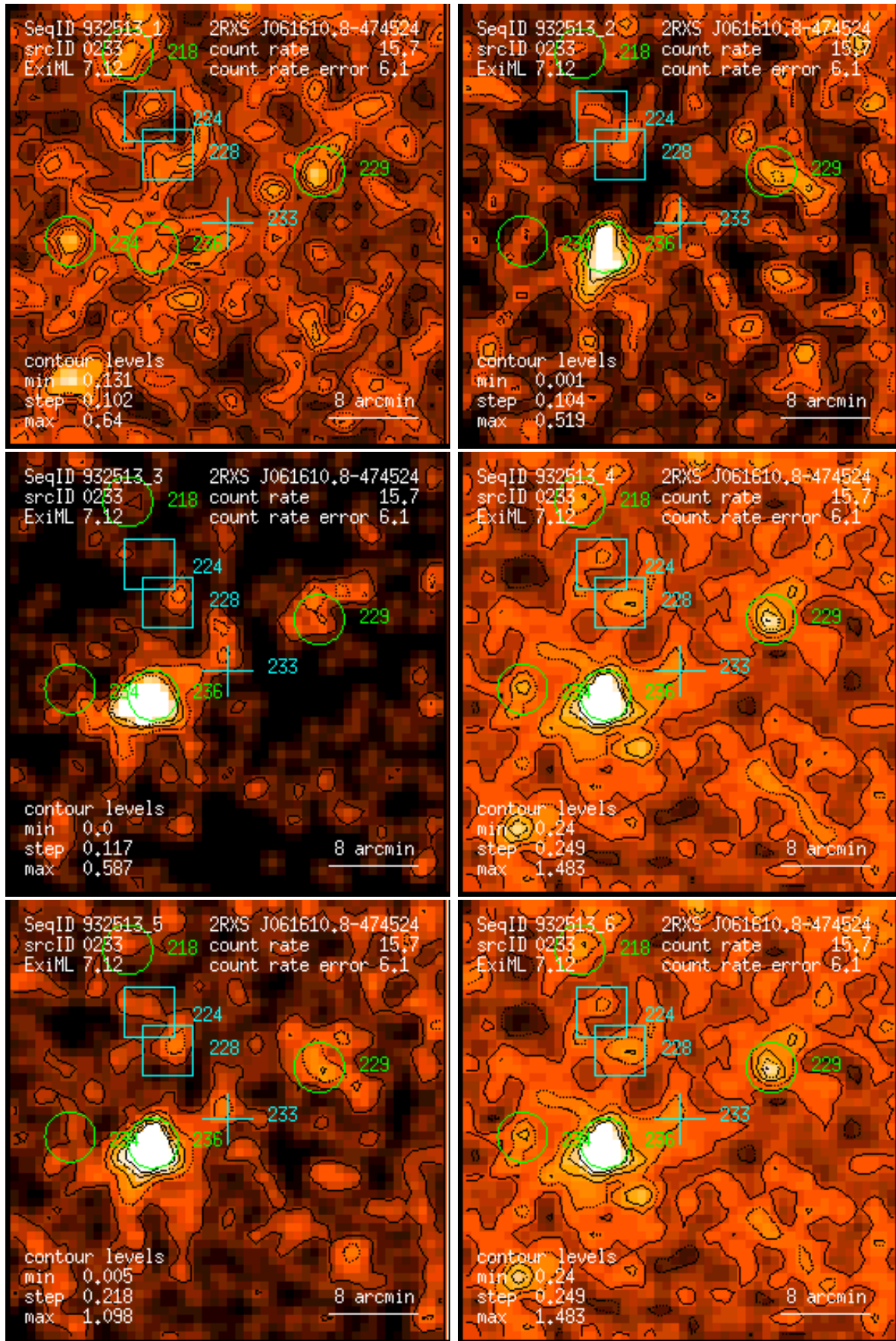
Figure 233: RASS 932513: detection 0233: band rate images, Gaussian filter: (1) PSPC channels 11 – 41, (2) 52 – 90, (3) 91 – 201, (4) 11 – 235, (5) 52 – 201, (6) 11 – 201. Broad band rates in counts/ks. Band rate contour levels in counts/ks/arcmin 2 .
