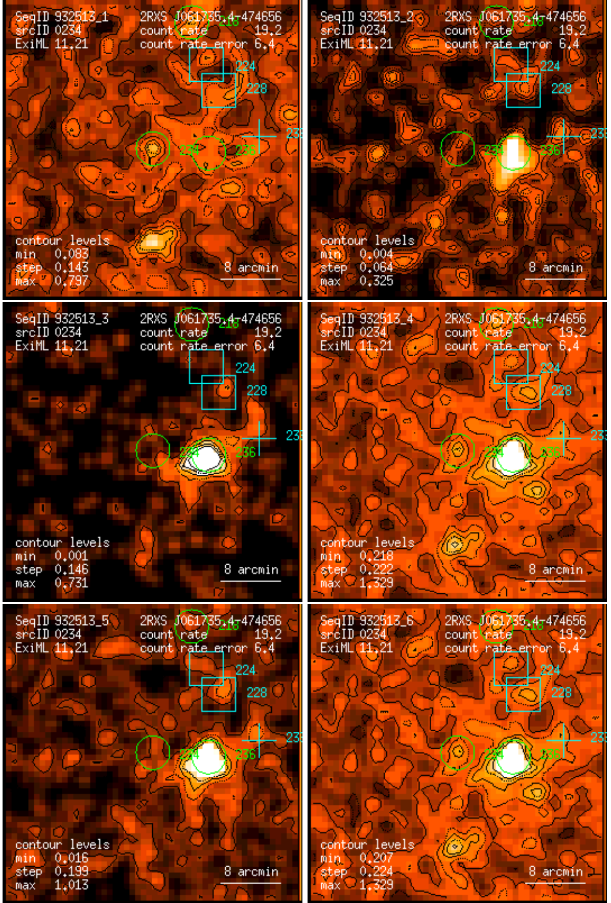
Figure 234: RASS 932513: detection 0234: band rate images, Gaussian filter: (1) PSPC channels 11 – 41, (2) 52 – 90, (3) 91 – 201, (4) 11 – 235, (5) 52 – 201, (6) 11 – 201. Broad band rates in counts/ks. Band rate contour levels in counts/ks/arcmin 2 .
