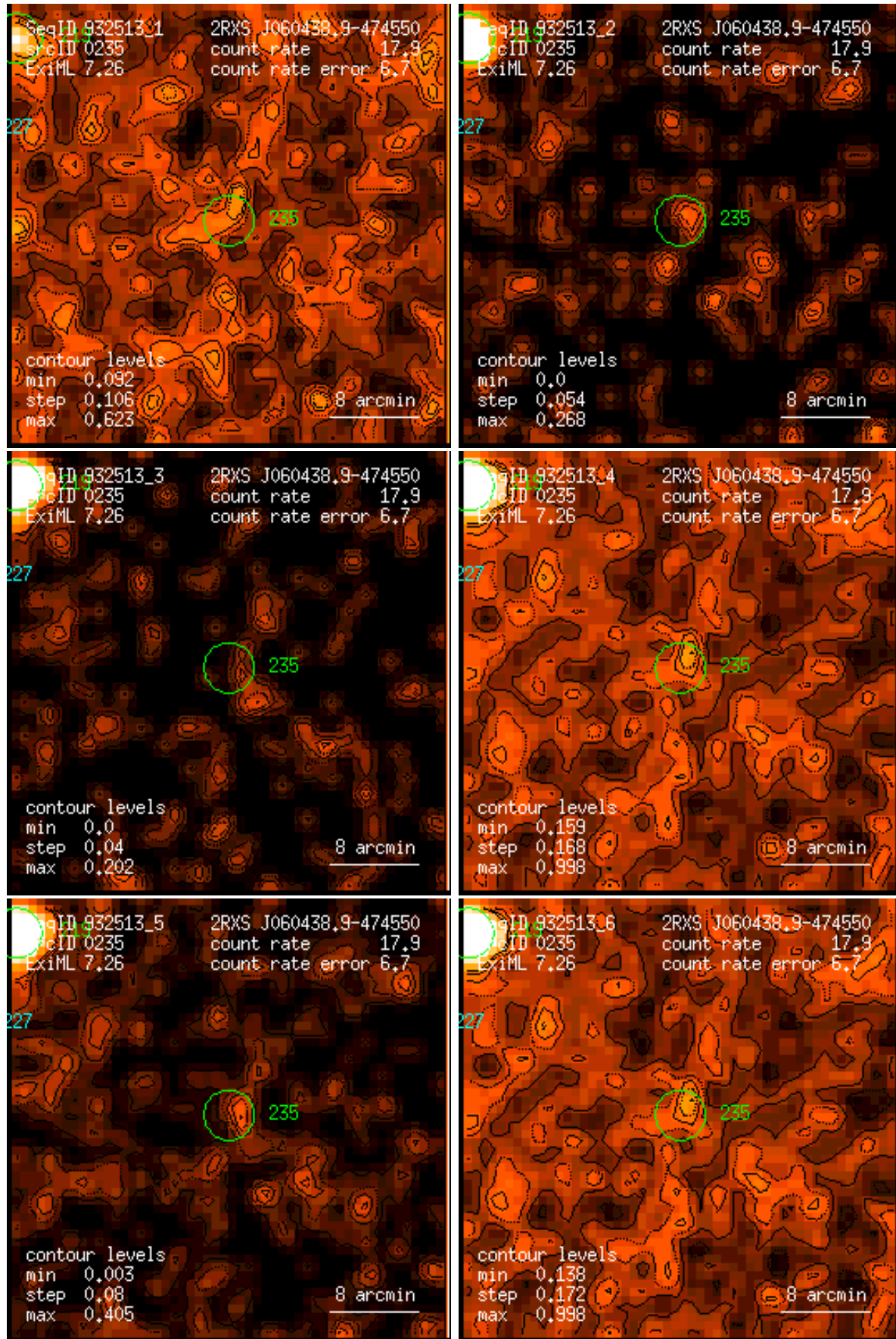
Figure 235: RASS 932513: detection 0235: band rate images, Gaussian filter: (1) PSPC channels 11 – 41, (2) 52 – 90, (3) 91 – 201, (4) 11 – 235, (5) 52 – 201, (6) 11 – 201. Broad band rates in counts/ks. Band rate contour levels in counts/ks/arcmin 2 .
